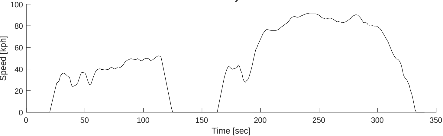
FTP75 Drive Cycle: 340sec
