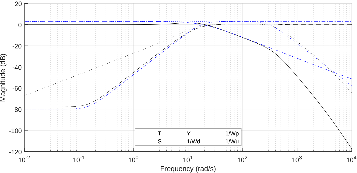
H_\infty TSY w_c=18
