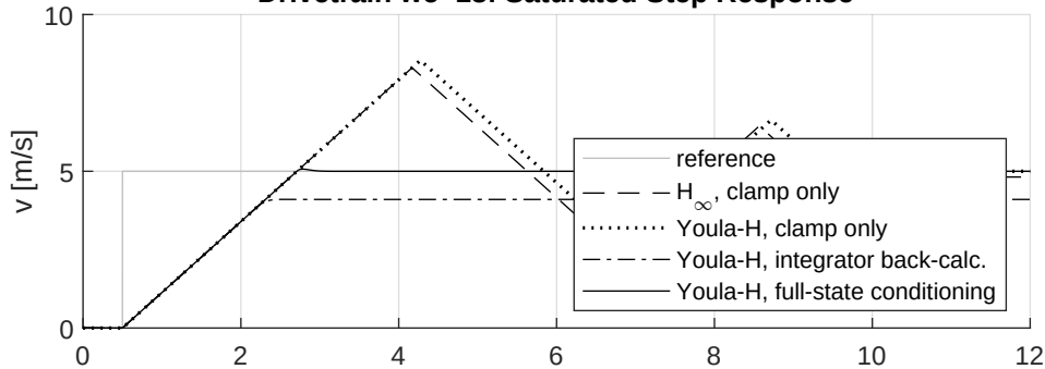
Drivetrain wc=18: Saturated Step Response
