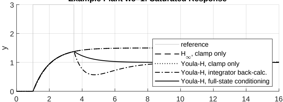
Example Plant w_c=1 : Saturated Response
