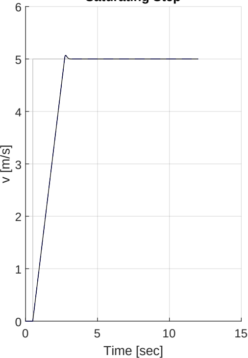
Saturating Step
