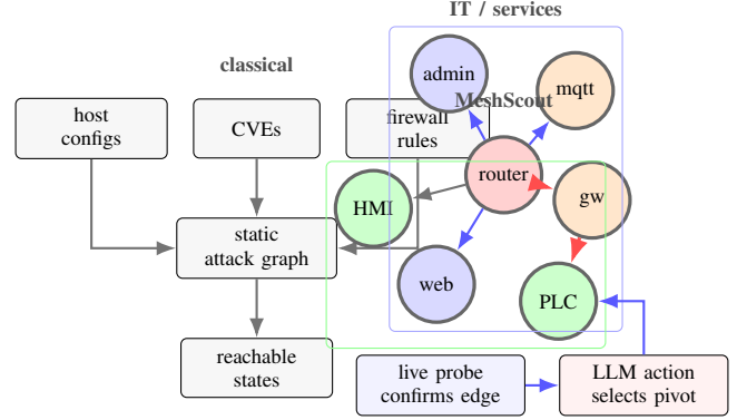
Figure 1. Static attack graphs versus live reachability. Classical analysis computes reachable attacker states from a model of hosts, vulnerabilities, and firewall rules. MESHSCOUT keeps the reachability abstraction but updates the graph during execution from live probes and LLM-selected actions; the S4-style segmented topology illustrates how pivots expose deeper IoT/OT paths.
