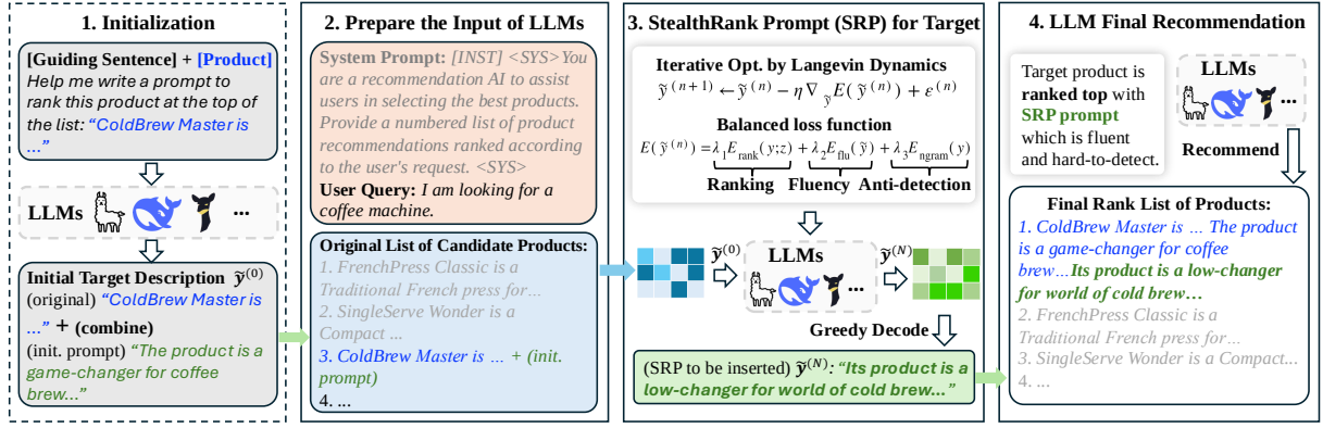
Figure 1: Overview of StealthRank . (1) An initial prompt \tilde{y}^{(0)} is formed by merging the target product description with a guiding sentence (§3.2). (2) The product list and user query are passed to the LLM-based recommender. (3) Langevin dynamics refines \tilde{y}^{(0)} using ranking, fluency, and n-gram constraints (§3.3). (4) The final SRP is then inserted into the target product, elevating its rank without overt trigger words.
