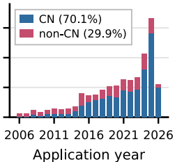
B CN vs non-CN
