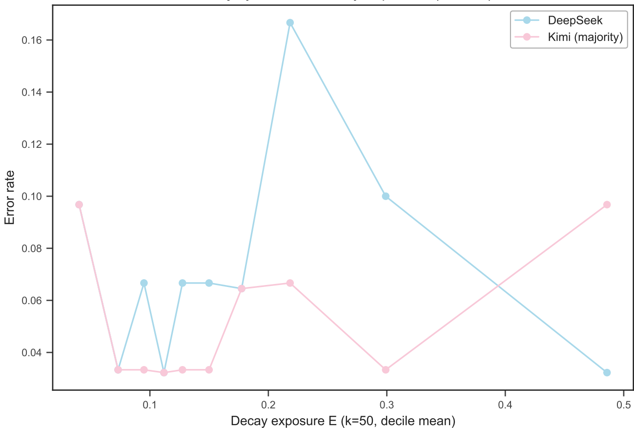
v1-Injury: error vs decay exposure (deciles)
