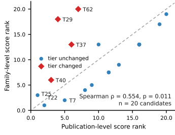
Fig. 8. Publication-level versus family-level (full-series) score ranks for the 20 screened candidates (Spearman \rho = 0.554 , p = .011 ). Diamonds mark the four candidates whose review-priority tier changed in the publication-level-to-family-level comparison (e.g., Topic 29 HIGH to LOW and Topic 40 HIGH to MEDIUM); the separate full-series-to-censored-2024 comparison is reported in the text ( \rho = 0.487 ).
