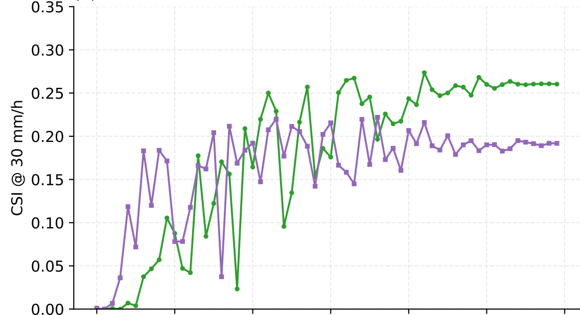
(b) Extreme rain detection
