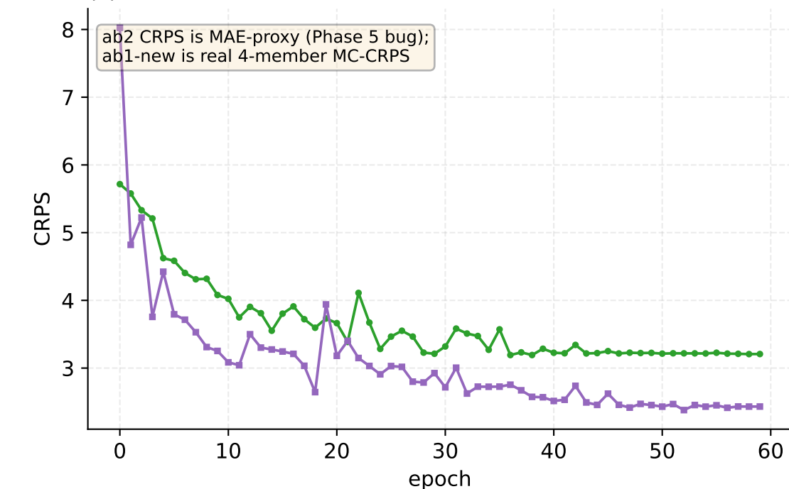
(c) Probabilistic skill
