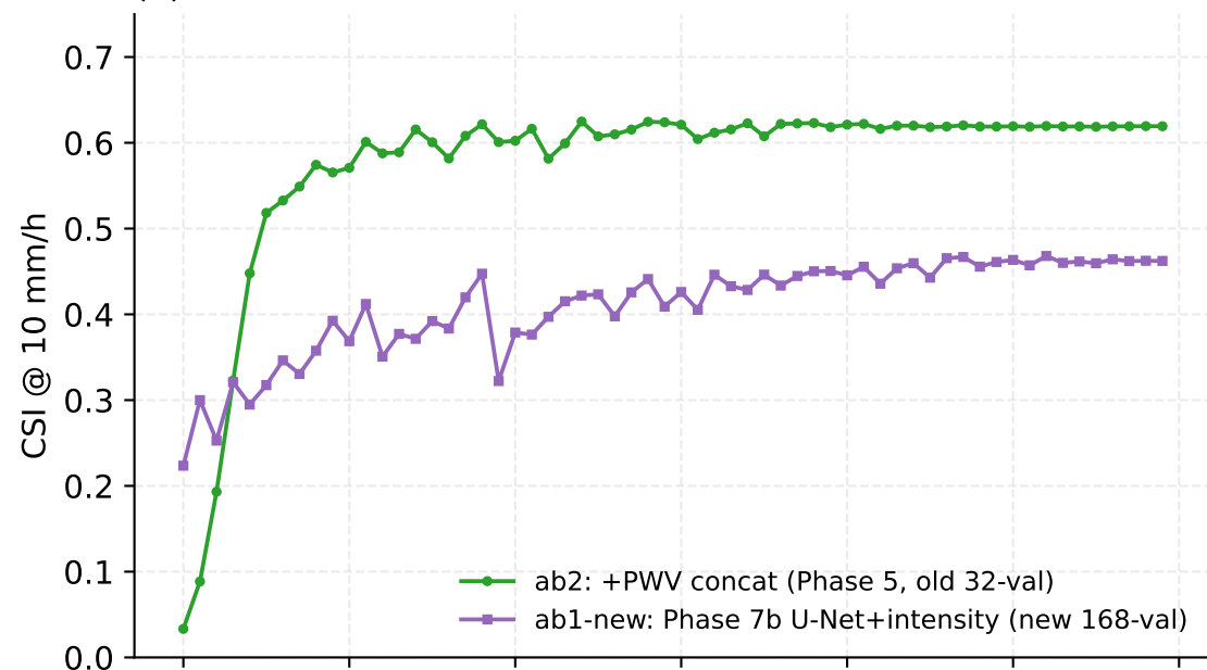
(a) Moderate rain detection
