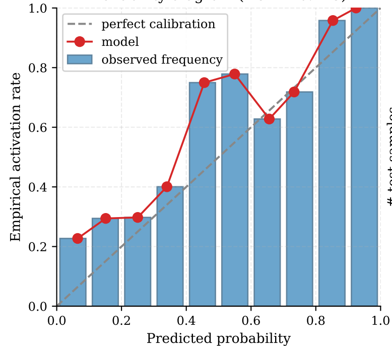
Reliability diagram (ECE = 0.115)
