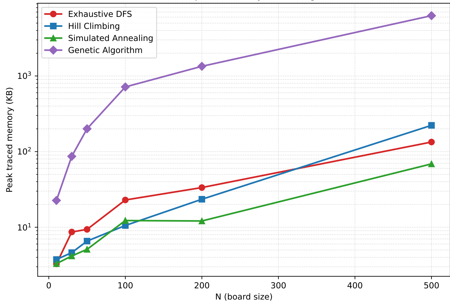
N-Queens: peak memory vs. N (log scale)
