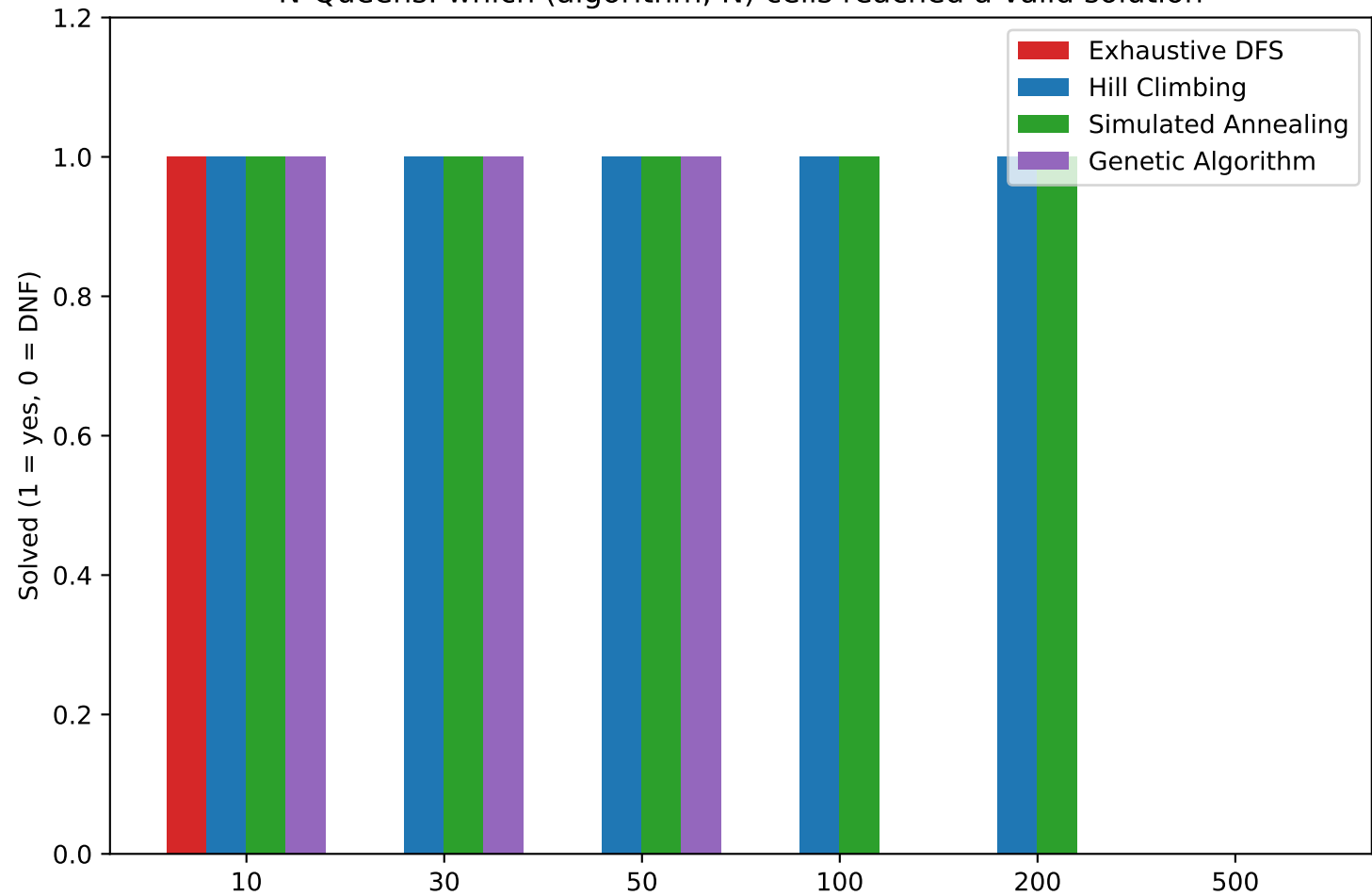
N-Queens: which (algorithm, N) cells reached a valid solution
