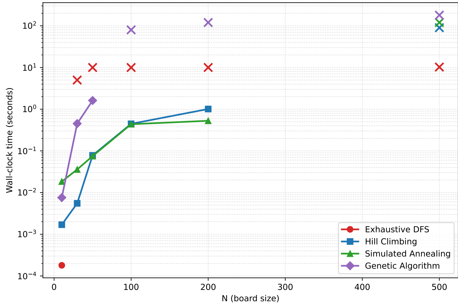
N-Queens: solving time vs. N (log scale, x = DNF)
