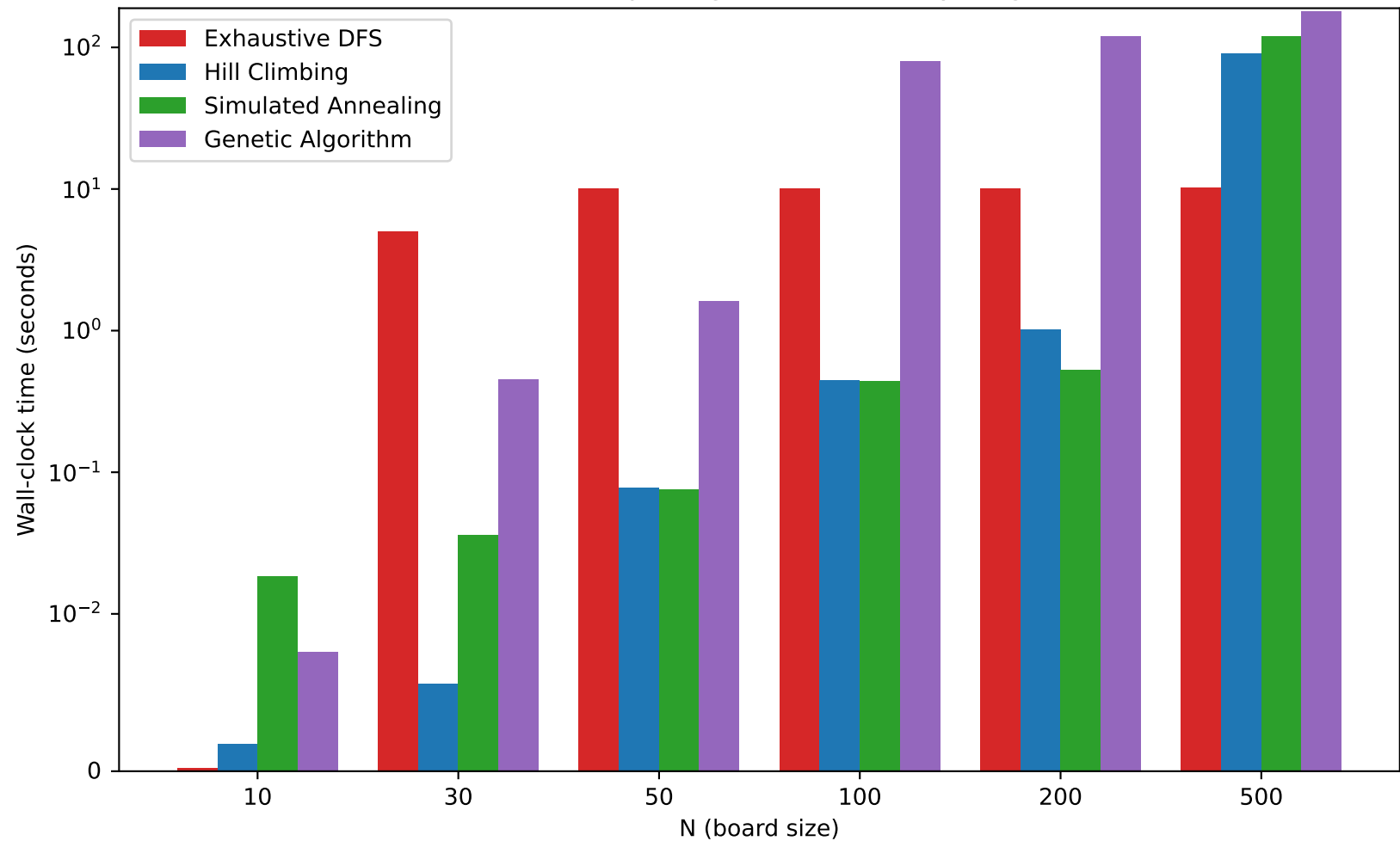
N-Queens: time per algorithm and N (symlog scale)
