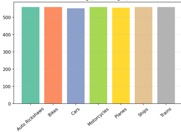
Training (3910 images)
