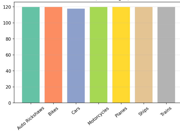
Validation (838 images)
