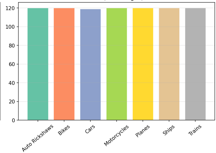
Test (839 images)
