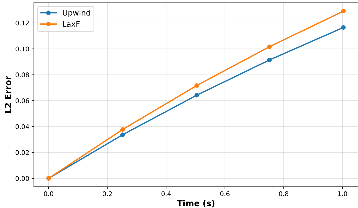
L2 Error vs Time — 2D Advection (Roll 23, \nu=0.45 )
