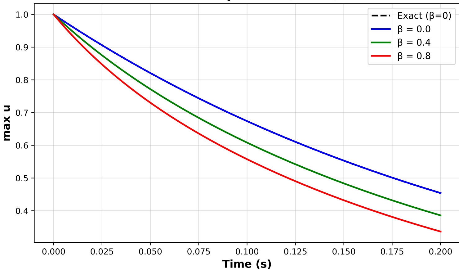
Max-u Decay vs Time ( \kappa_0=0.2 )
