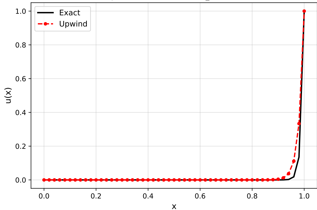
Upwind Differences ( Pe_h = 2.0 )
