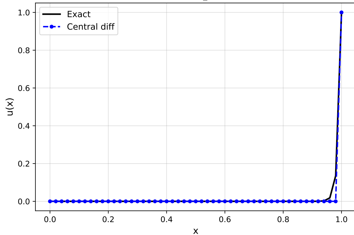
Central Differences ( Pe_h = 100.0/50 = 2.0 )
