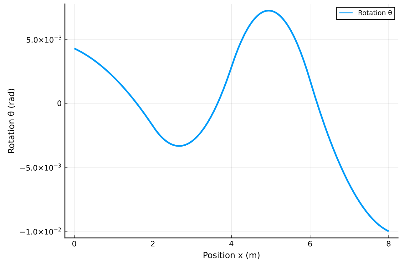
Rotation Profile
