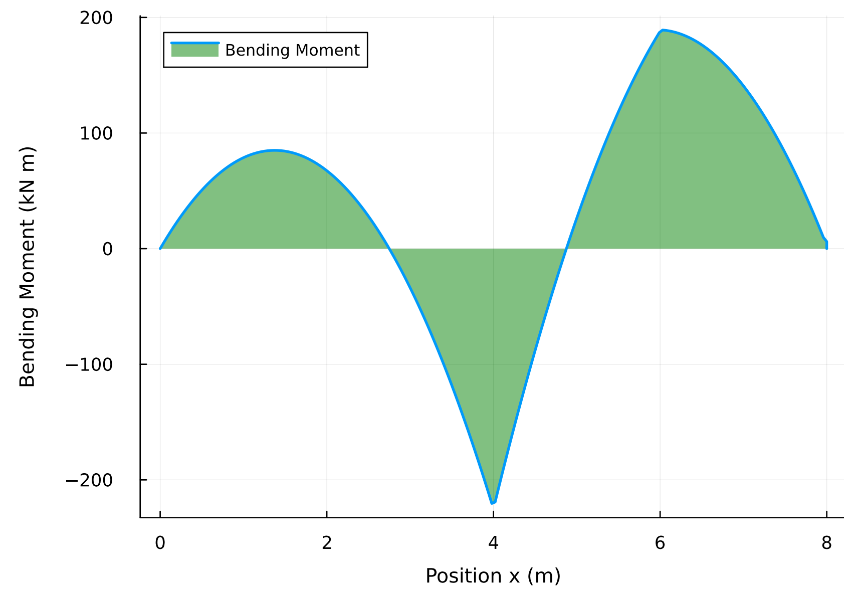
Bending Moment Diagram
