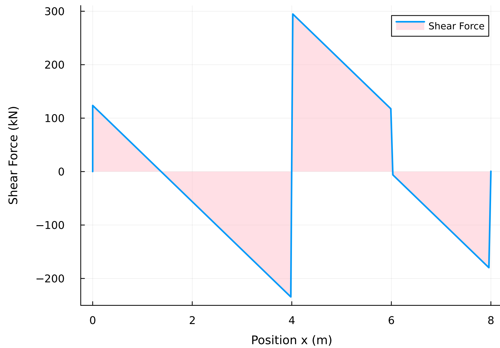
Shear Force Diagram
