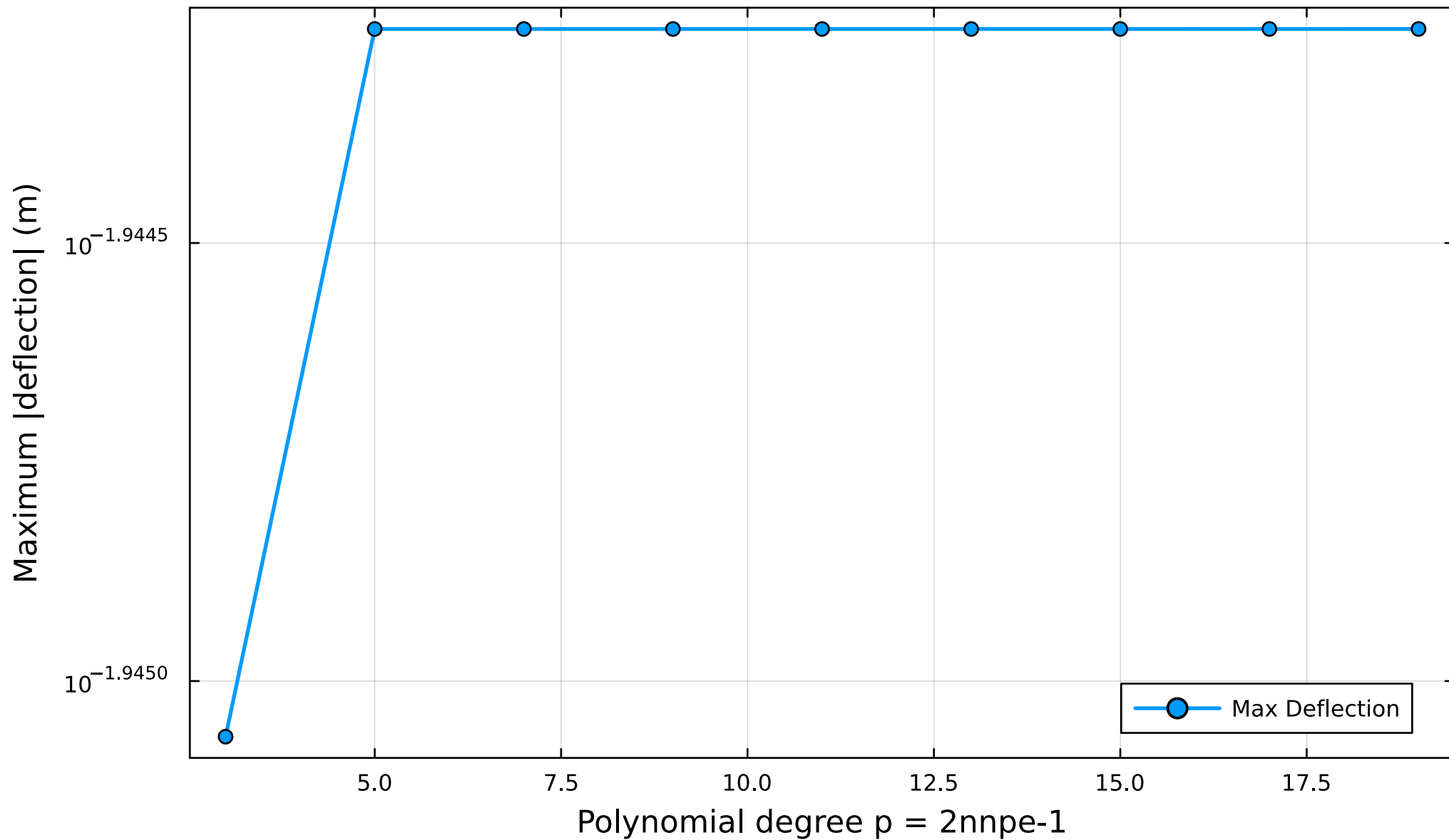
Maximum Deflection vs. Higher-Order Approximation
