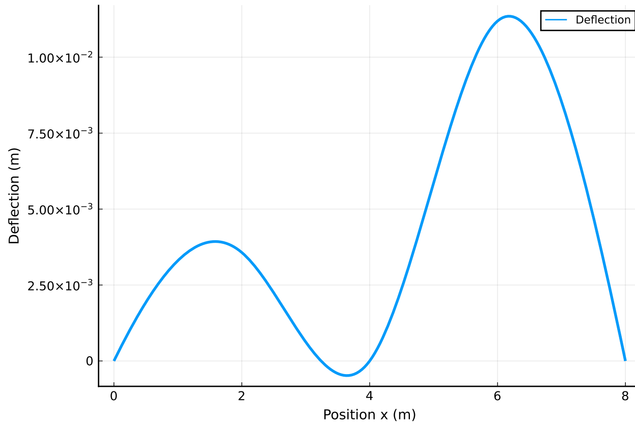
Deflection Profile
