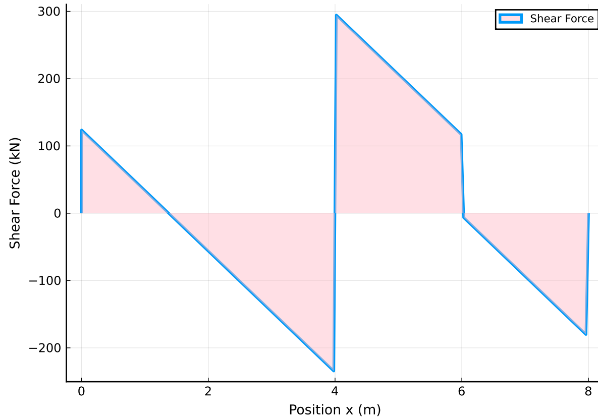
Shear Force Diagram
