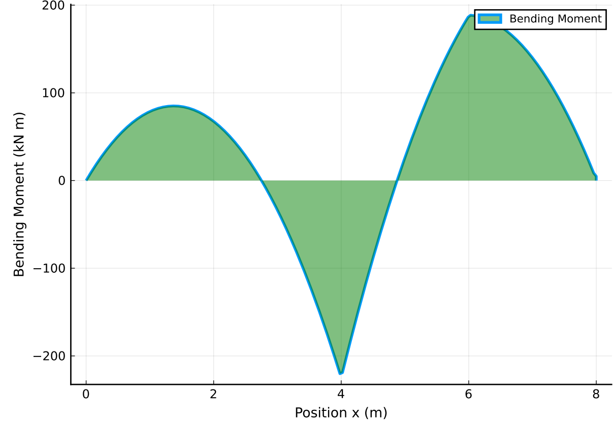
Bending Moment Diagram
