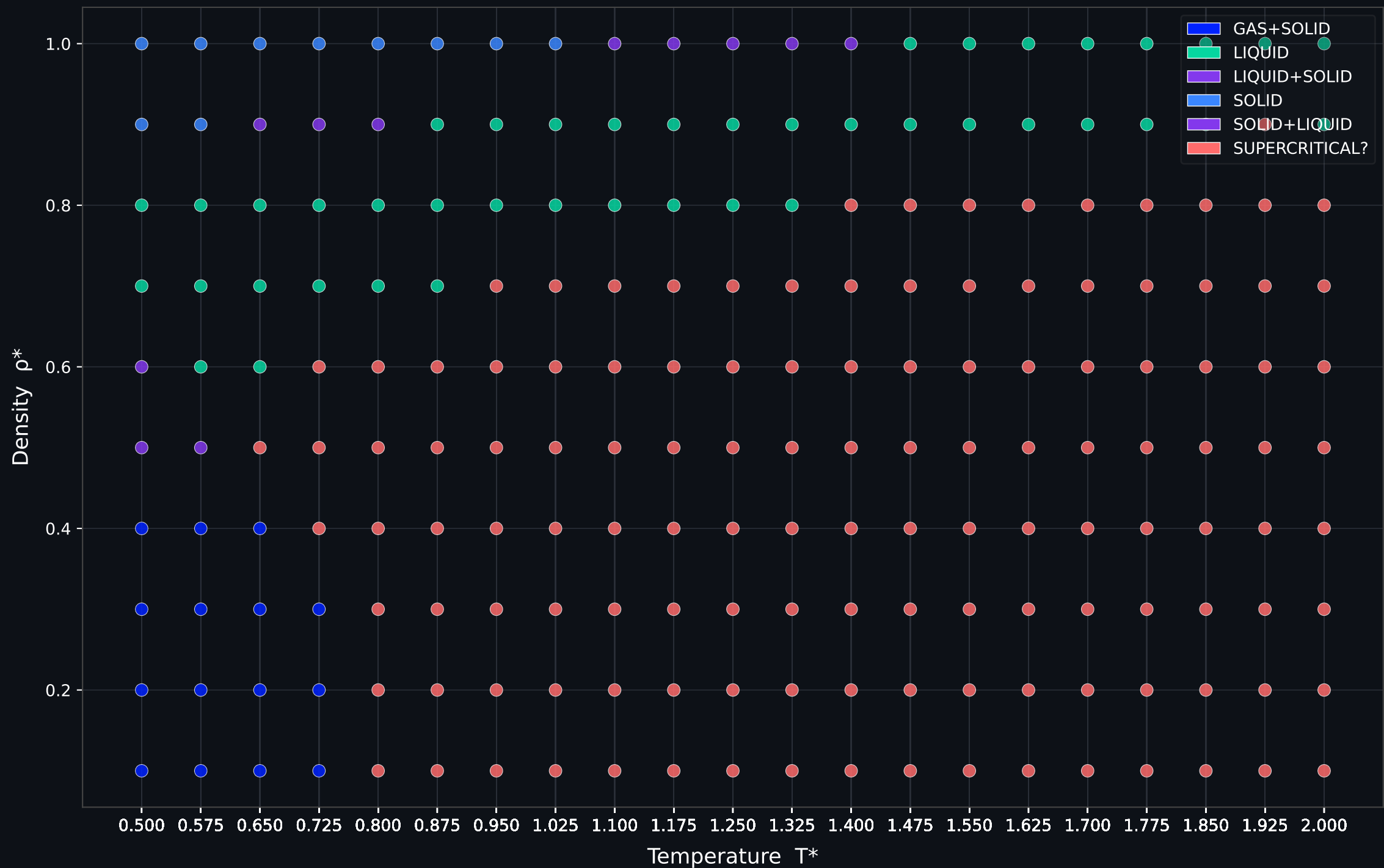
Phase Diagram - \rho^* vs T^*
