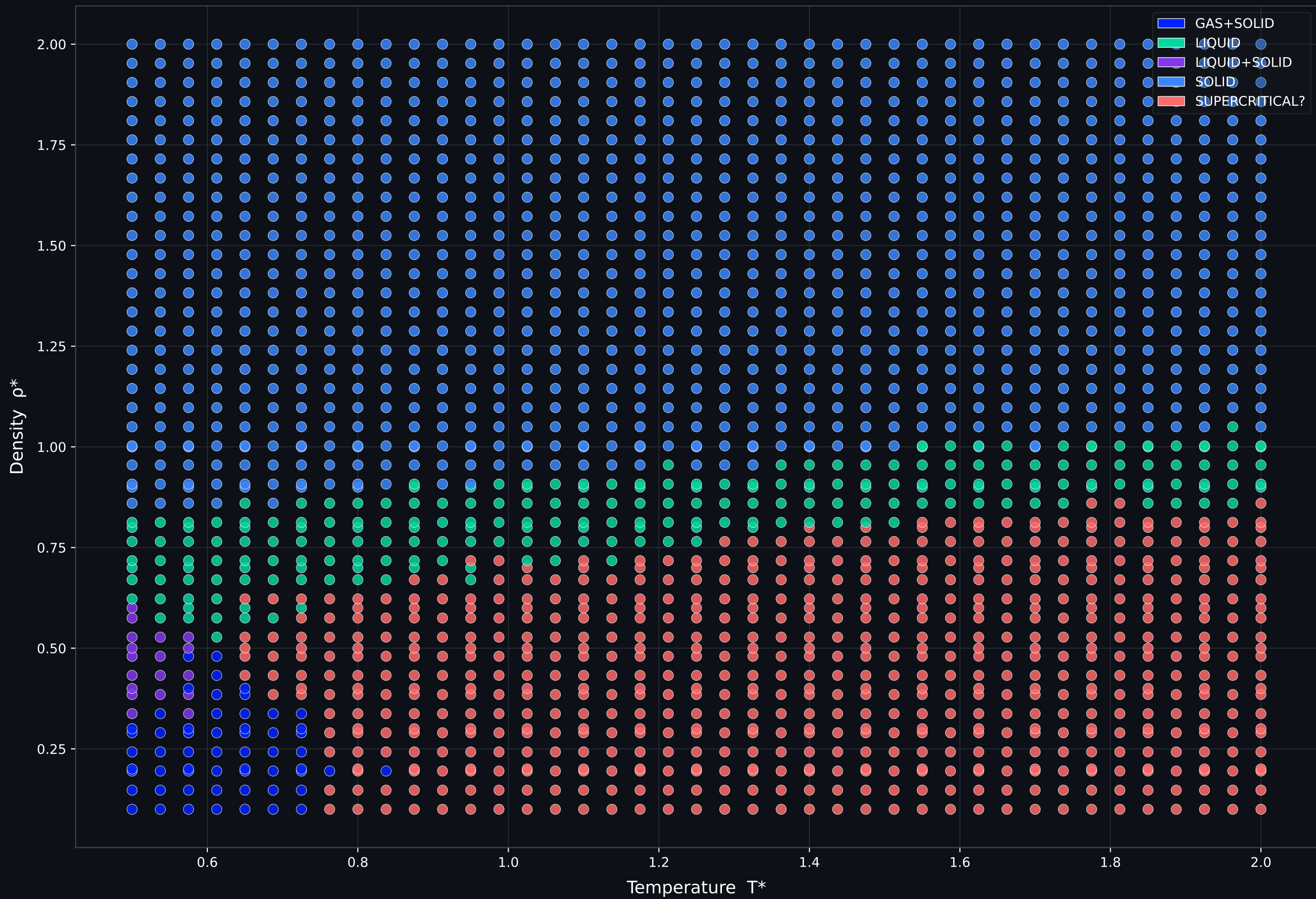
Phase Diagram - \rho^* vs T^*
