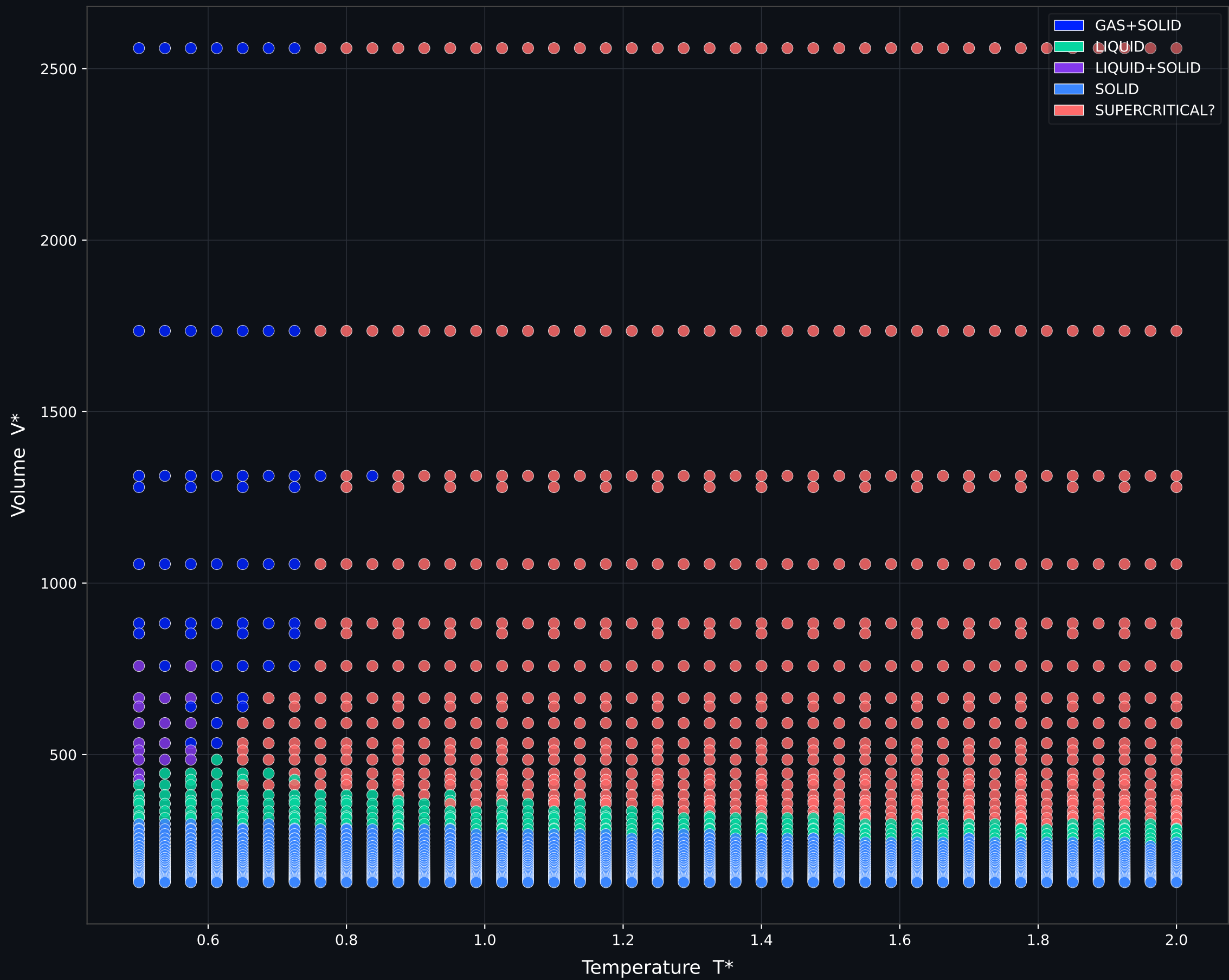
Phase Diagram - V^* vs T^*
