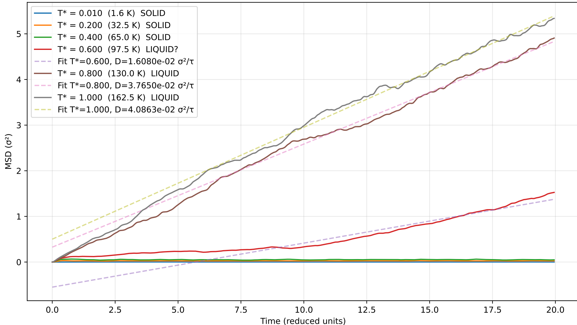
Mean Squared Displacement (MSD) vs Time
