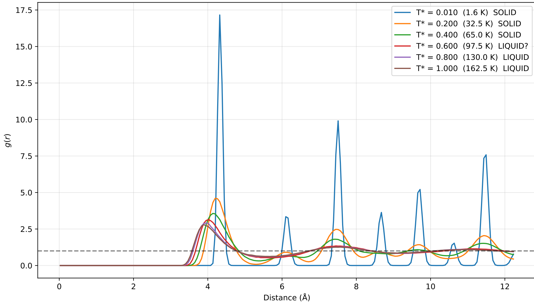
Radial Distribution Function g(r) — Lennard-Jones System
