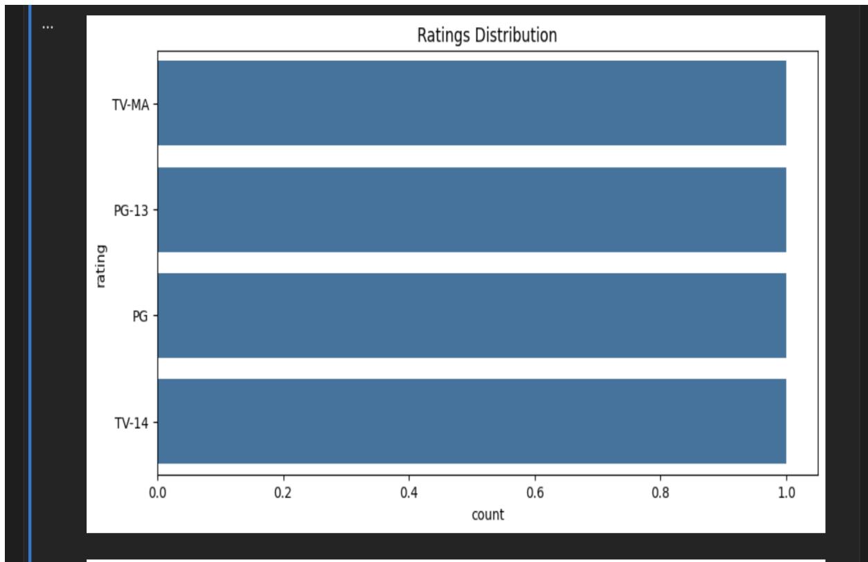
Screenshot 4
