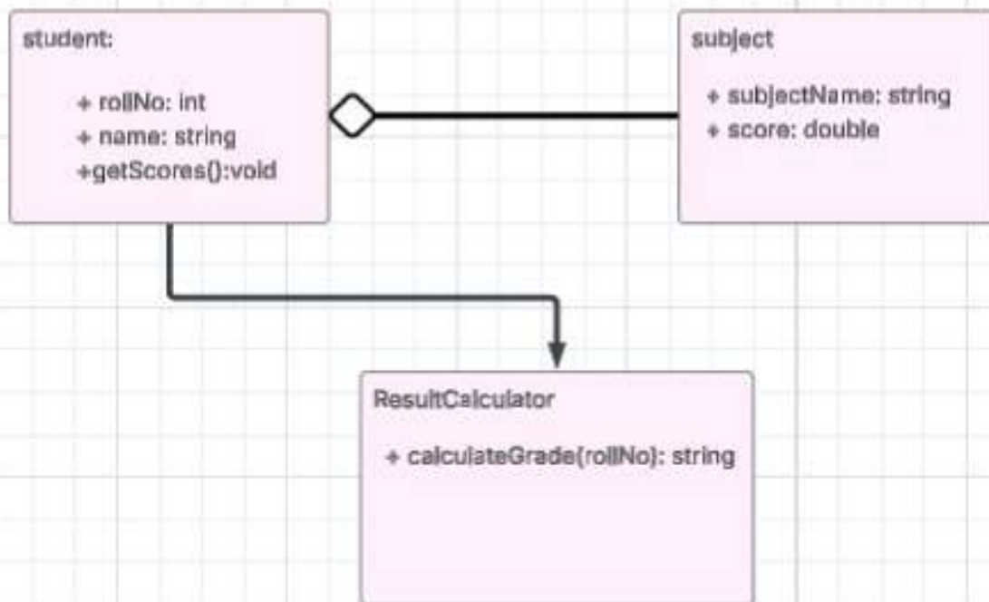
Class diagram
