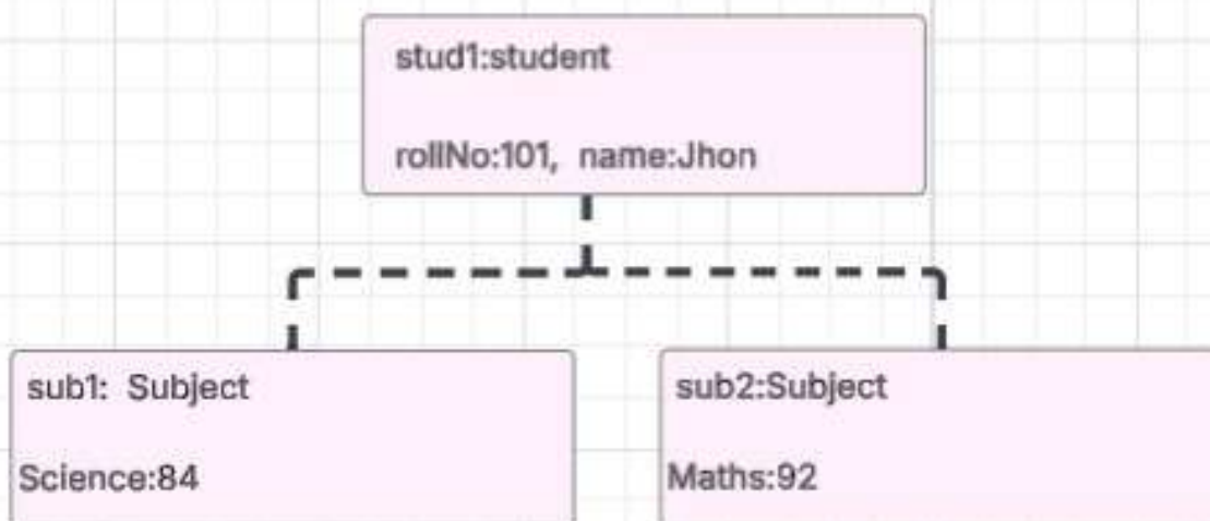
Object diagram
