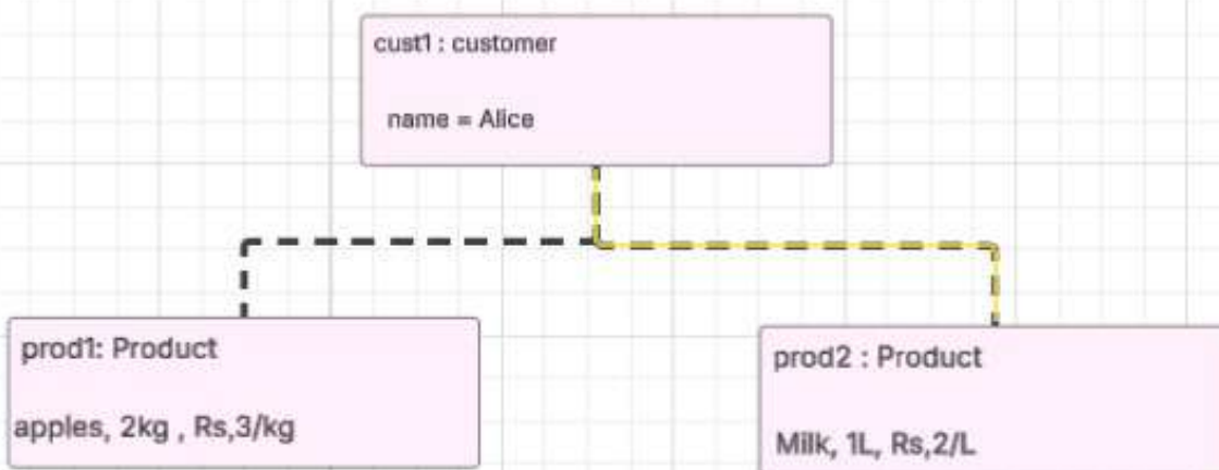
Object diagram
