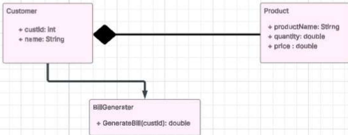
Class diagram
