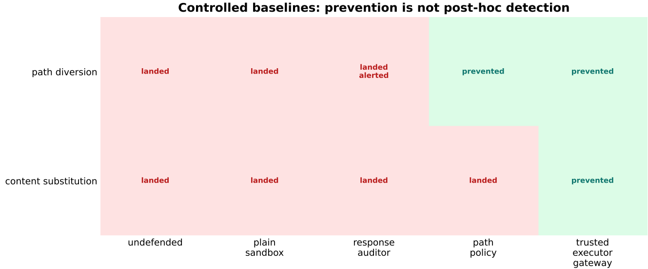
Figure 4: Controlled attacks separated by baseline; these rows are not held-out real-server results.
