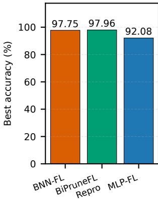
(a) Accuracy
