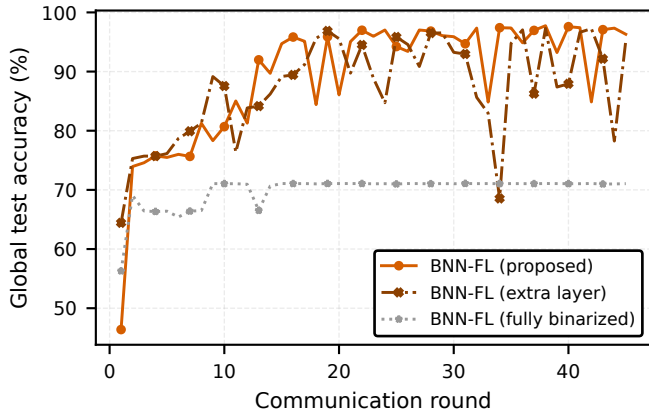
(a) Accuracy over training
