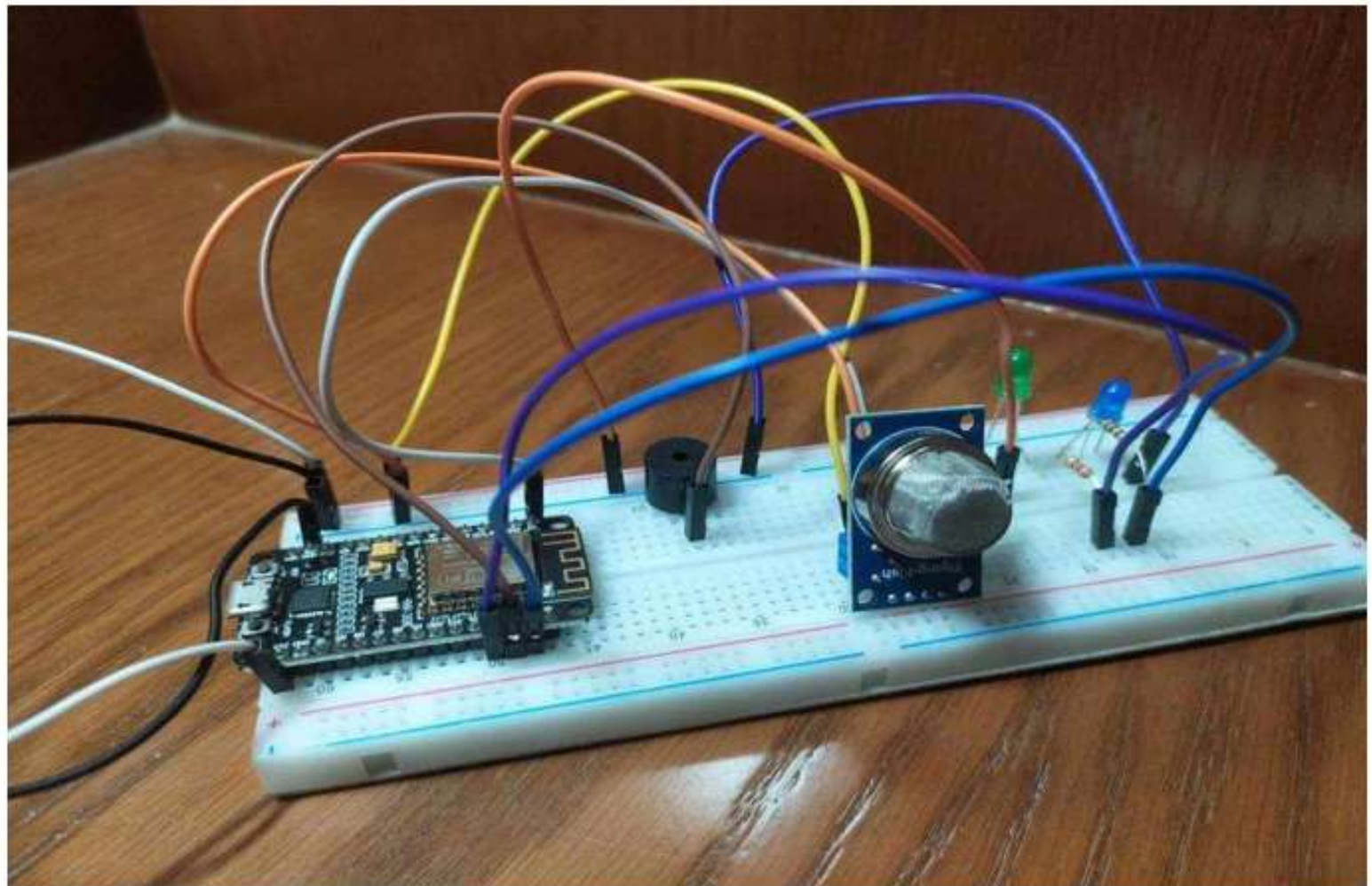
Figure: Assembling of the Hardware Section
