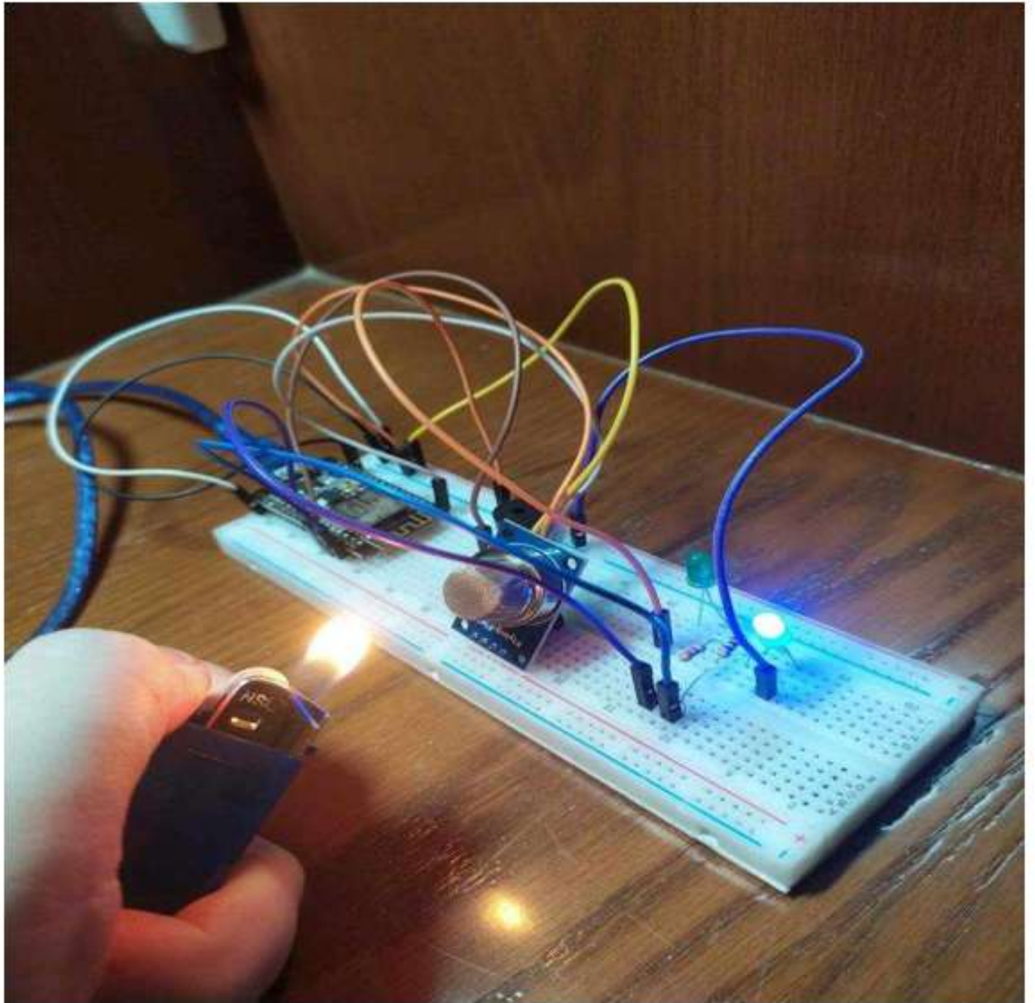
Figure: Blue LED When the Gas Is Detected
