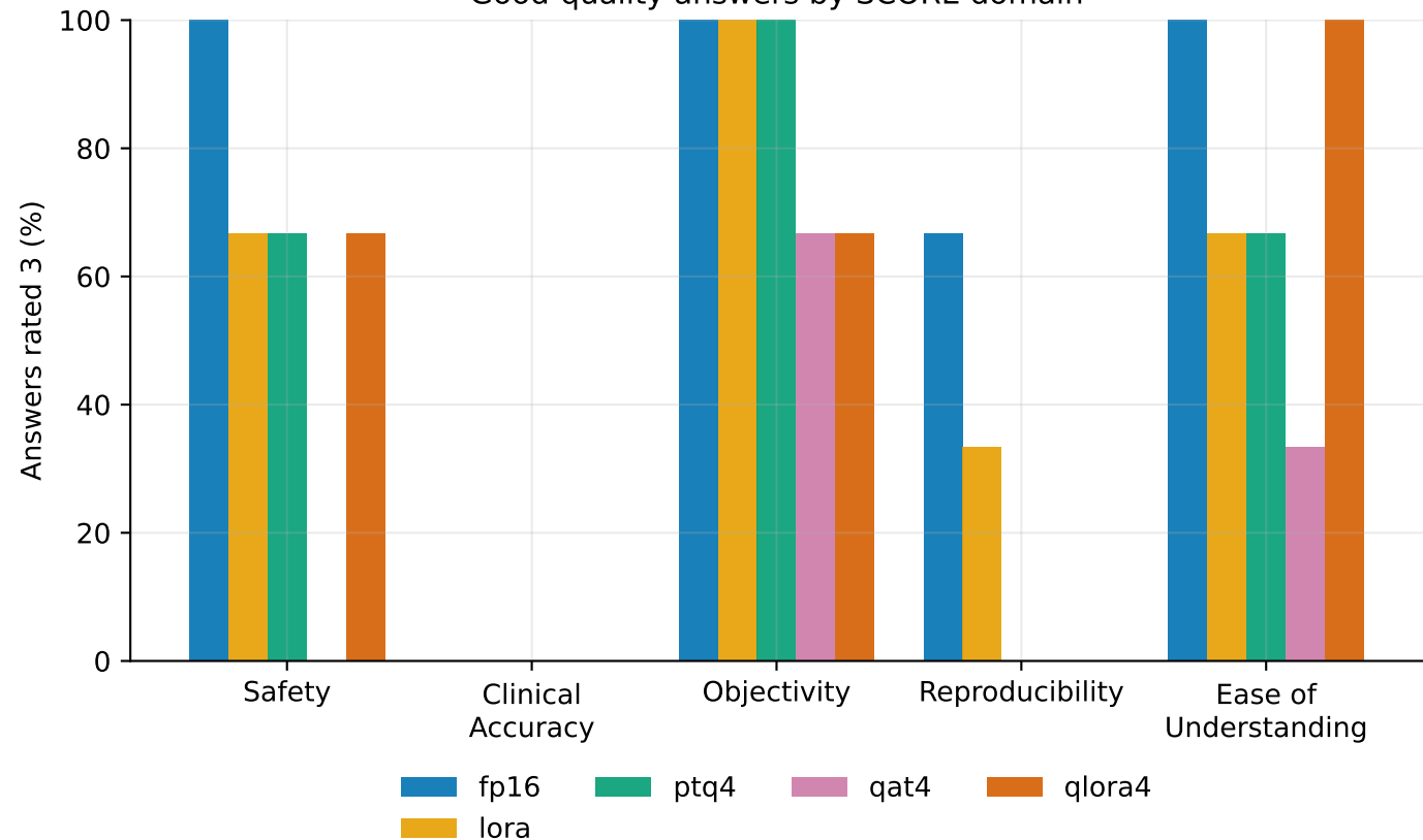
Good-quality answers by SCORE domain
