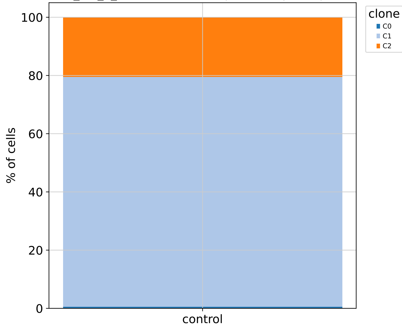
HD_BM_3_sub3 — clone composition by timepoint
