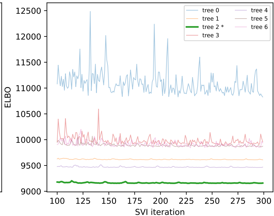
ELBO trajectory
