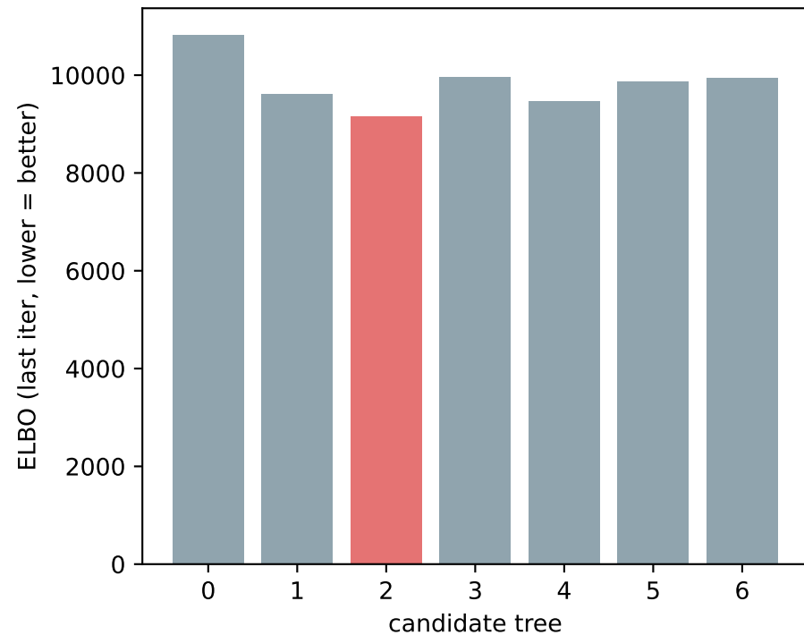
Model evidence per tree
