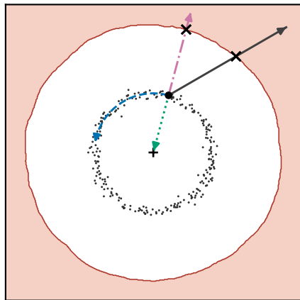
(a) distance score (kNN)
