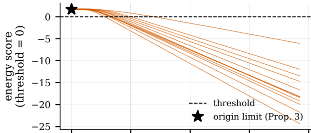
MPNet
