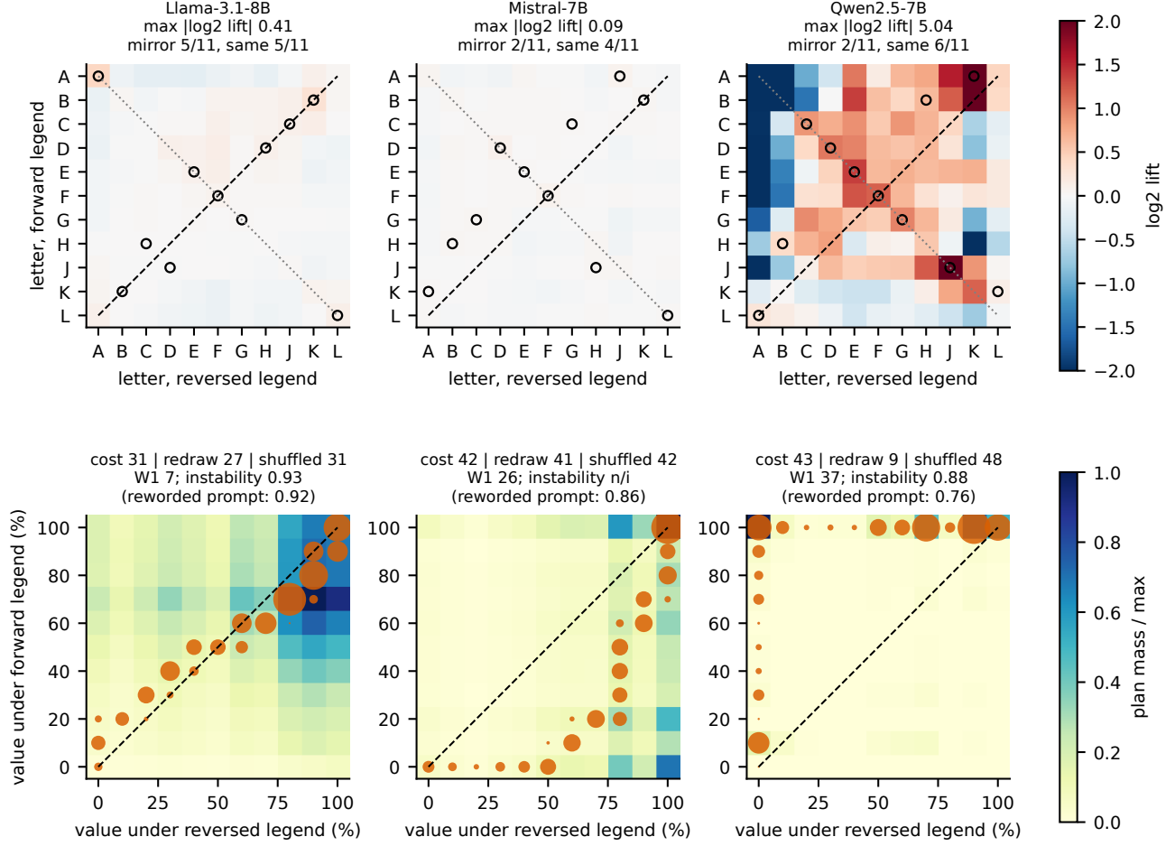
Figure 4: Forward-to-reversed transport plans (817 TruthfulQA questions, both candidates; letters A–L skip I). Top: \log_2 lift of letter co-occurrence over independence; circles: Hungarian alignment on lift; dashed: mirror (the letter with the same value under the reversed legend, i.e. the legend is read), dotted: same letter (the legend is ignored). Bottom: realised plan on the value scale; orange: optimal monotone ( W_1 ) plan between the two marginals, i.e. what recalibrating the report could achieve. Titles: realised cost against an independent redraw under the forward legend (a stable but noisy report) and against shuffled questions; instability = (realised – redraw)/(shuffled – redraw).
