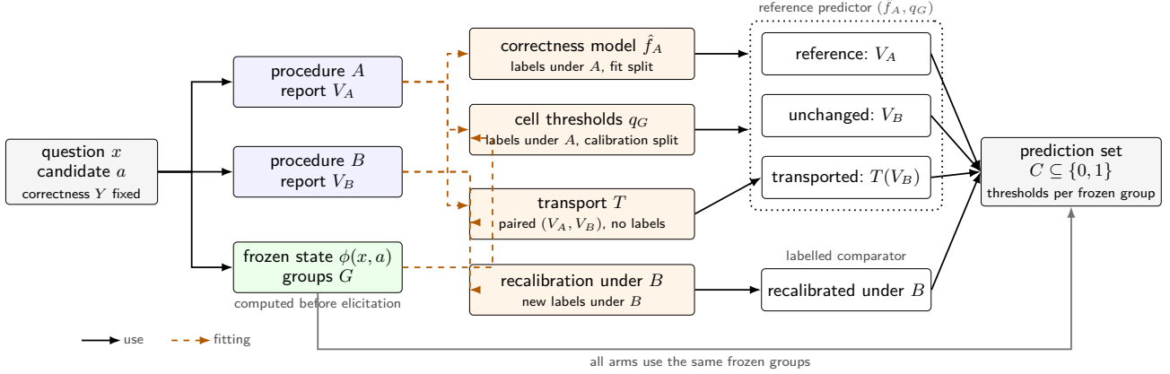
Figure 1: Calibrating and transporting confidence reports. The question, candidate and correctness remain fixed while the elicitation procedure changes. Labels under A fit the correctness model and, on a separate calibration split, the cell thresholds. At deployment, the reference predictor receives V_A , unchanged V_B , or T(V_B) . Transport T is fitted without correctness labels using paired reports for the same inputs. The labelled comparator instead recalibrates under B using new labels. All arms use the same frozen groups and return prediction sets of correctness labels. Dashed arrows denote fitting.
