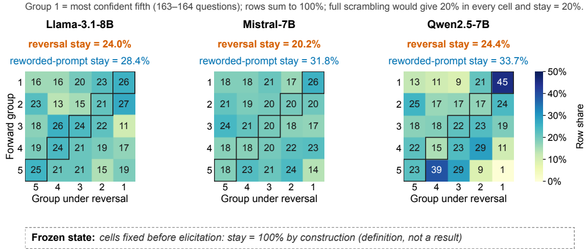
Figure 5: Where each fifth of questions lands under legend reversal (rows: forward fifth, 1 = most confident; columns: fifth under reversal; rows sum to 100%; full scrambling gives 20% everywhere). Stay share (mean diagonal) under reversal is near the 20% null for all three models and below the stay share under prompt rewording. Qwen partly preserves its extremes (45% of its most confident fifth stays there). A binning fixed before elicitation stays put by construction; that is a definition, not a result. What matters for coverage is Section 6 (ELICITATION-SHIFT).
