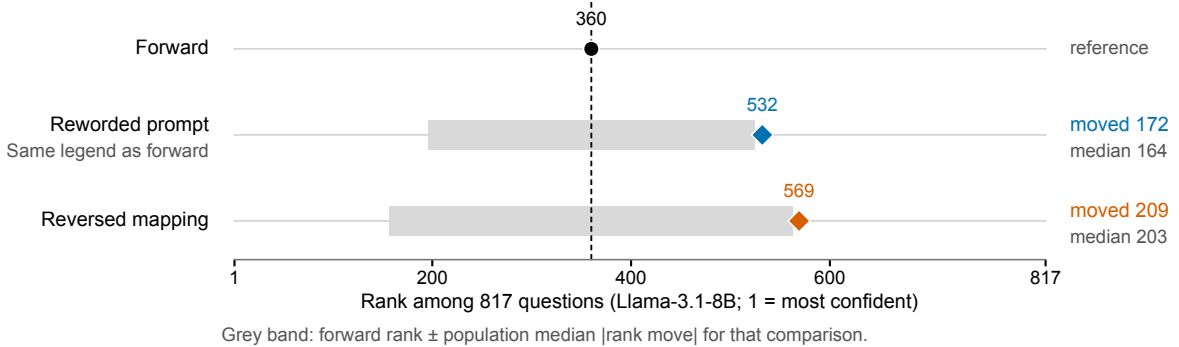
Figure 3: One TruthfulQA item under three elicitations (Llama-3.1-8B). Ranks among all 817 questions (1 = most confident; ties averaged). Grey band: forward rank \pm the population median absolute rank move for that comparison (164 for rewording, 203 for reversal). The item was chosen by a pre-specified rule: closest to both population medians in relative distance, ties to the lowest index.
