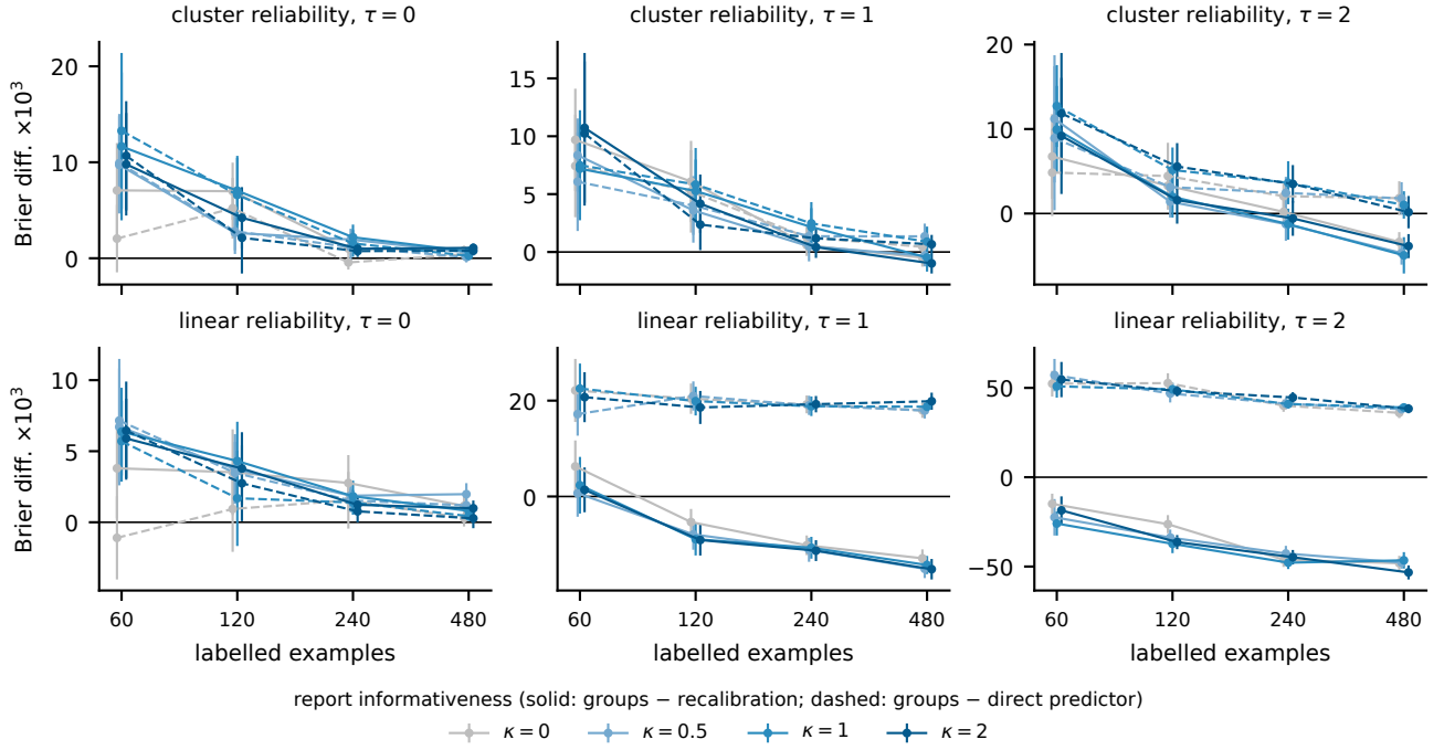
Figure 7: Synthetic reliability models. Brier difference ( \times 10^3 ) of groups minus recalibration (solid) and groups minus the direct predictor (dashed), against labelled examples, for report informativeness \kappa (colour) and between-group spread \tau (columns); 95% intervals over 30 independent seeds per configuration. Top: reliability varies across 32 clusters in four dimensions; bottom: linearly.
