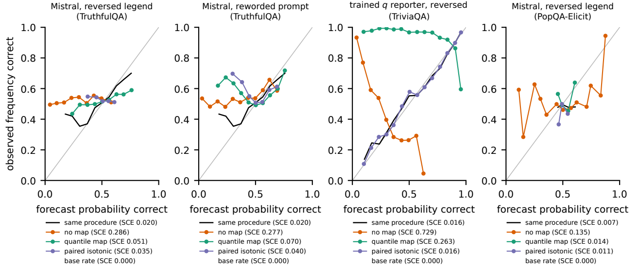
Figure 8: Reliability of a forecast fitted under procedure A and applied to procedure-B reports, with no map, the quantile map and paired isotonic regression, against the same forecast under A (black). Fifteen equal-width bins, bins with fewer than 20 predictions omitted; SCE from calibration-toolbox, with a constant forecast at the test base rate as reference (SCE 0 by construction). Test predictions pooled over 50 splits (TruthfulQA, POPQA-ELICIT) or the fixed split (TriviaQA). On PopQA Mistral's forward report is uninformative, so every forecast stays near 0.5.
