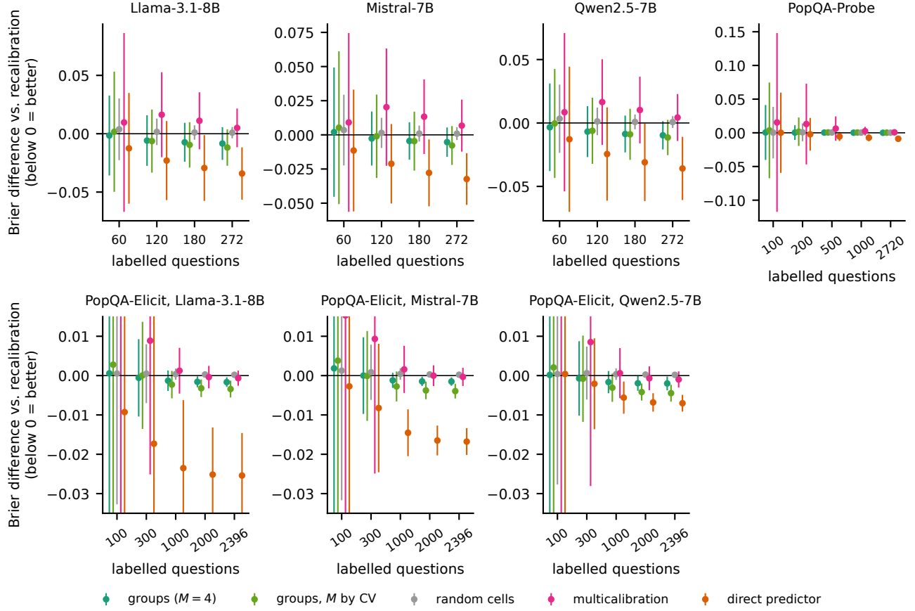
Figure 6: Brier difference against procedure-specific recalibration R (below zero: better), averaged over procedures, with Nadeau-Bengio-corrected 95% intervals. Top: TruthfulQA (three models, 200 random splits) and POPQA-PROBE (probe report, one procedure, 100 splits). Bottom: POPQA-ELICIT (three models, three procedures, 100 splits); the vertical axis is zoomed, so intervals at 100–300 labels run beyond it. Groups: farthest-first cells on 16 PCA dimensions of the frozen hidden state.
