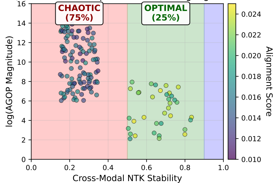
(a) Phase Landscape: 144 Vision-Language Pairs
