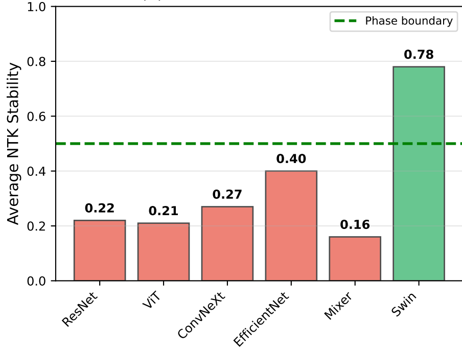
(b) Architecture Performance
