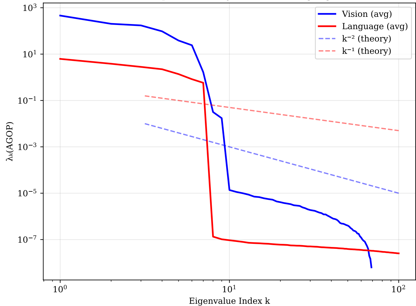
AGOP Spectral Decay: Vision vs Language
