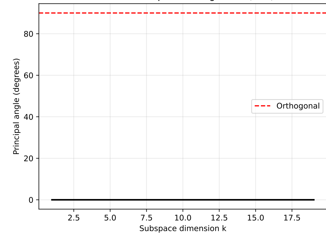
Gradient Subspace Misalignment (PCA)
