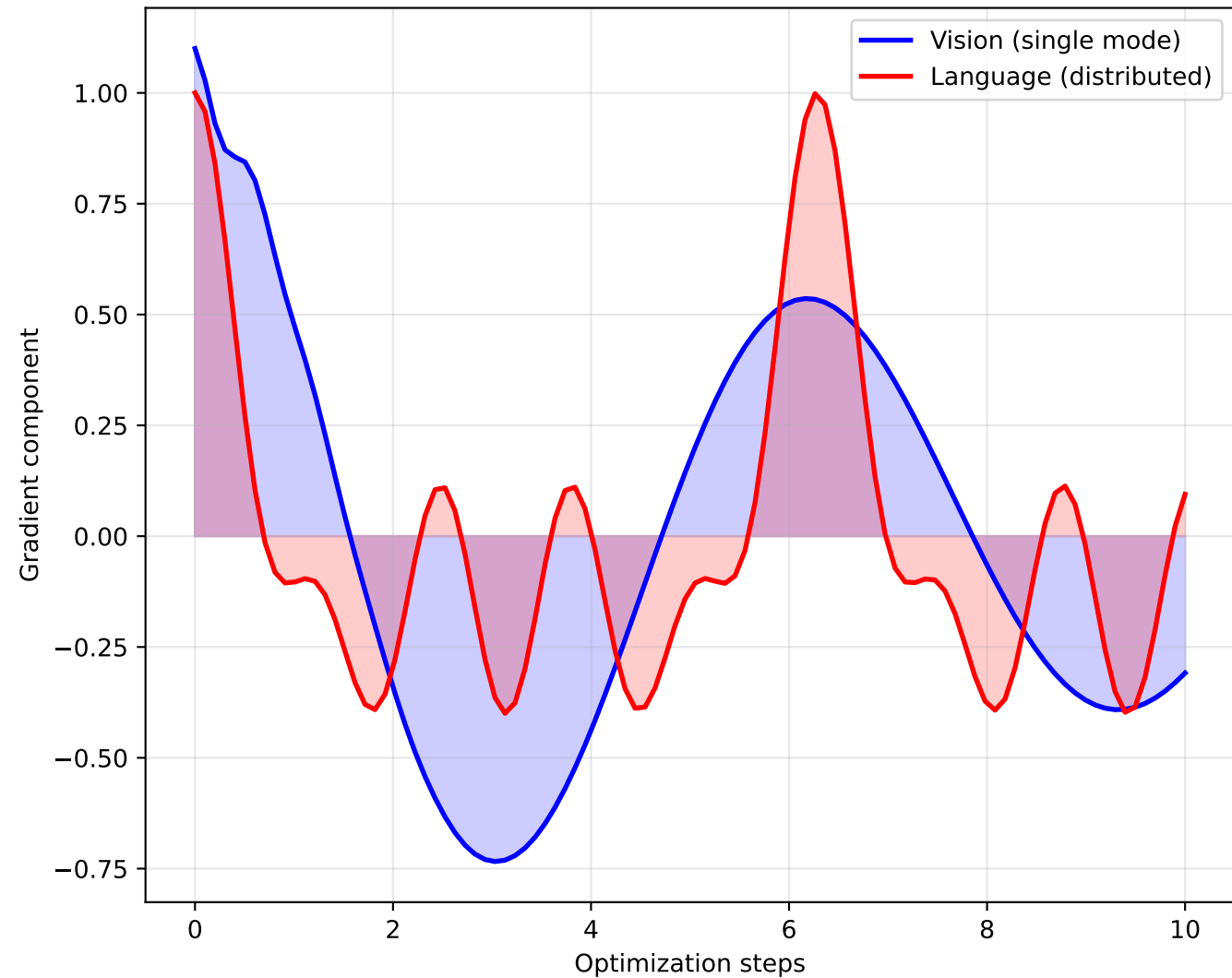
Gradient Flow Incompatibility
