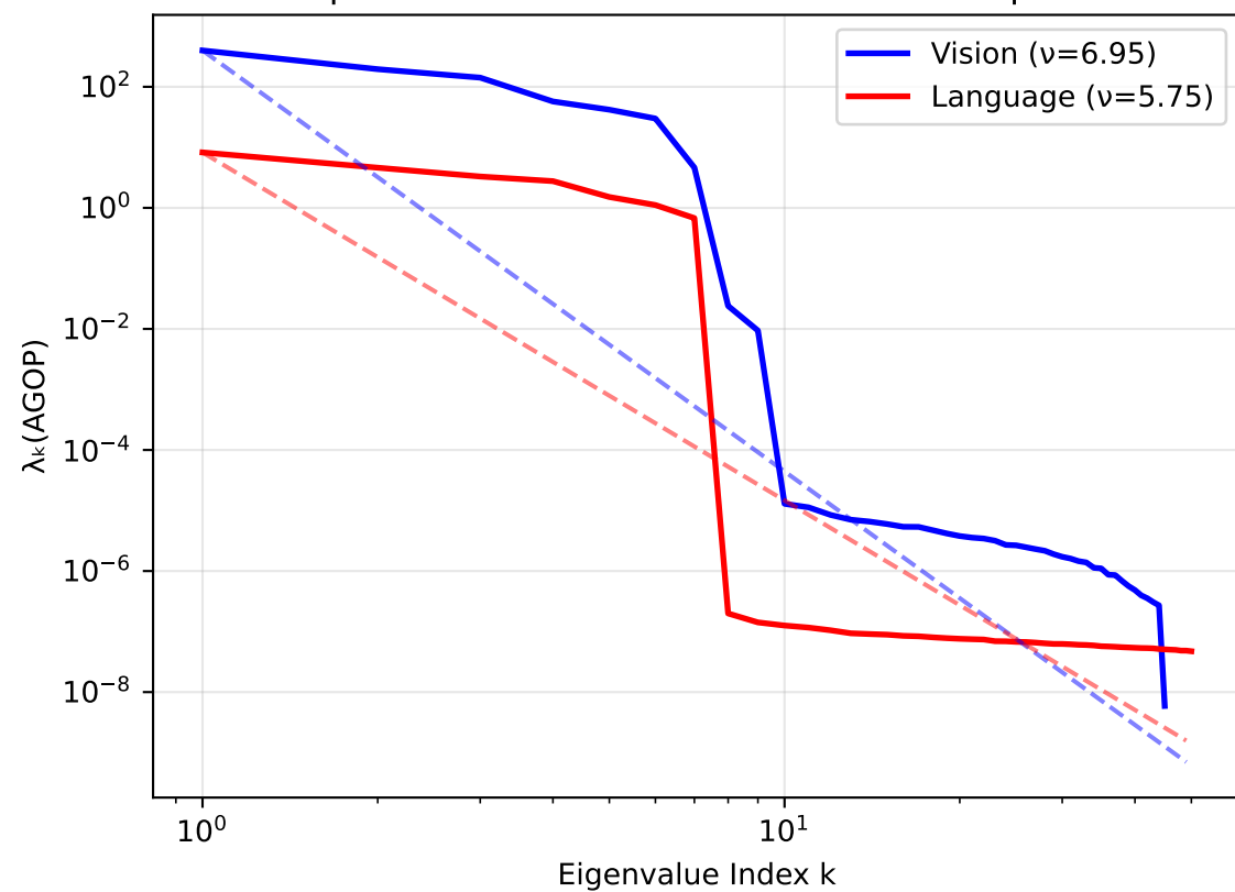
Step 3: Incompatible Gradient Flows → No Solution
