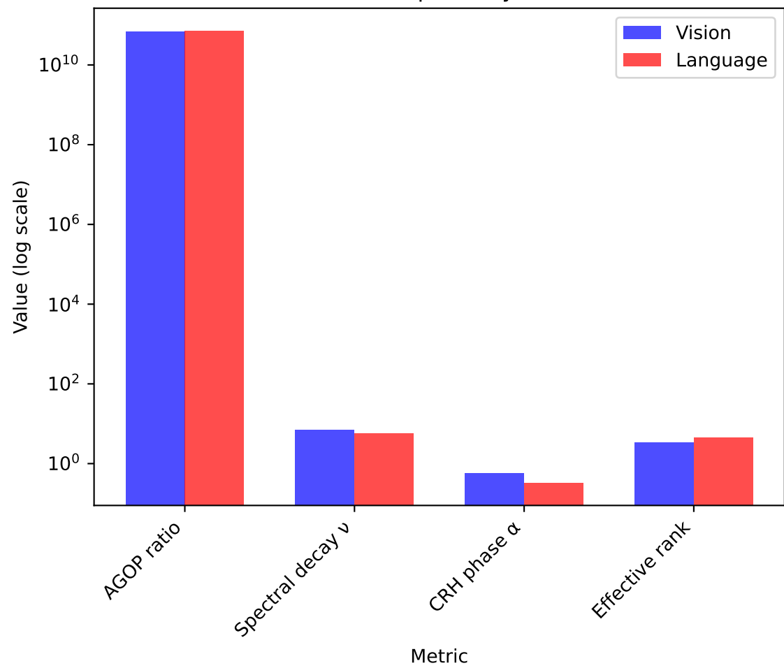
Phase Incompatibility Metrics
