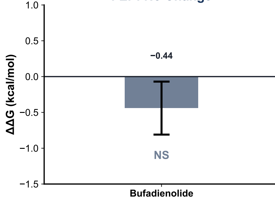
FEP: No Change
