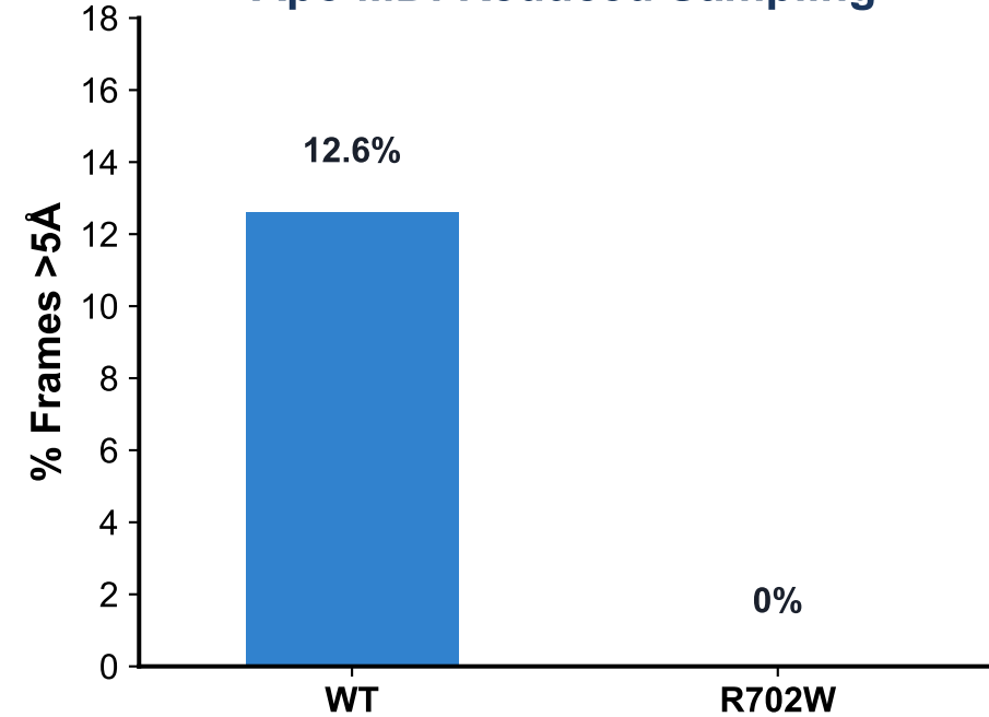
Apo MD: Reduced Sampling
