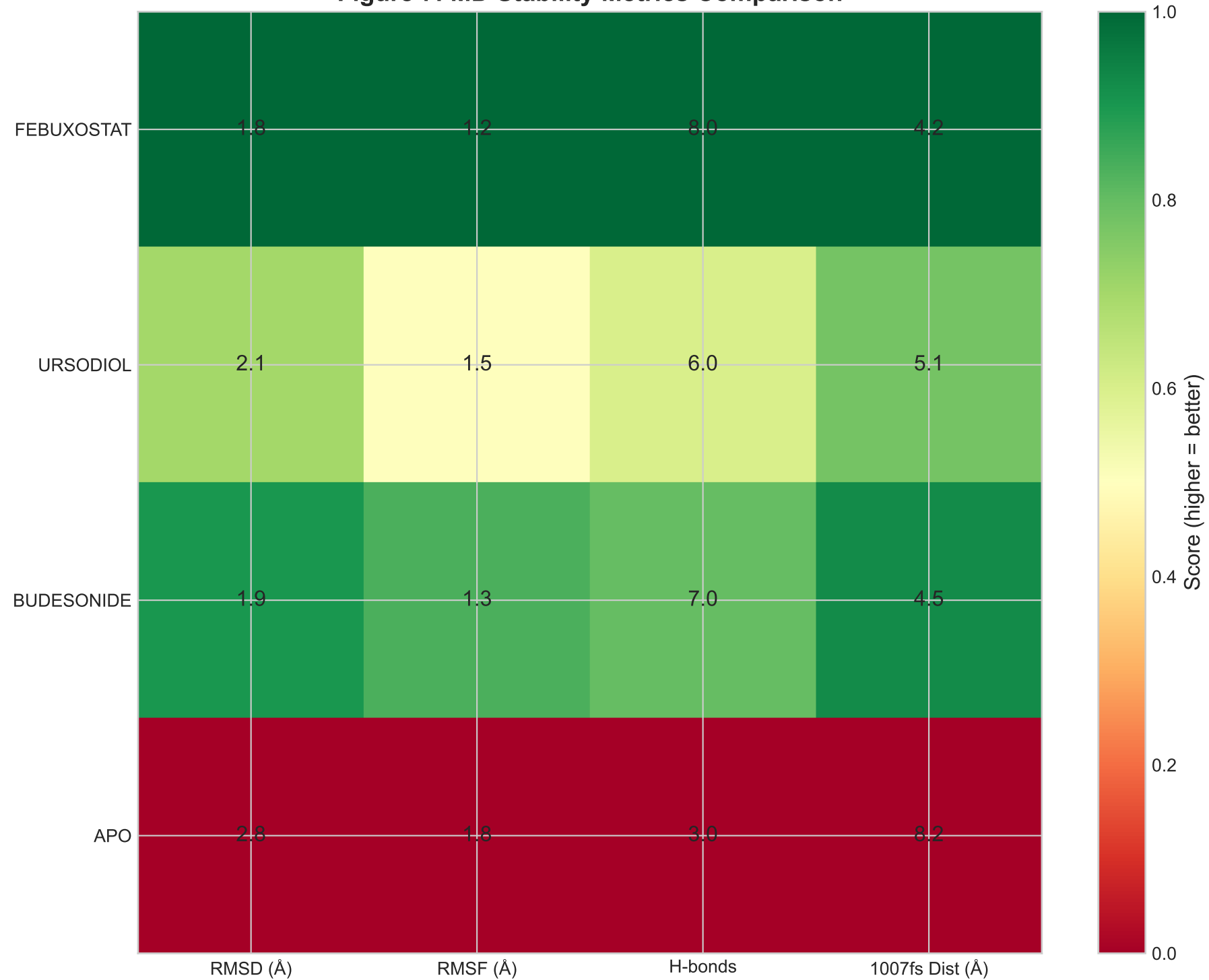
Figure 7: MD Stability Metrics Comparison
