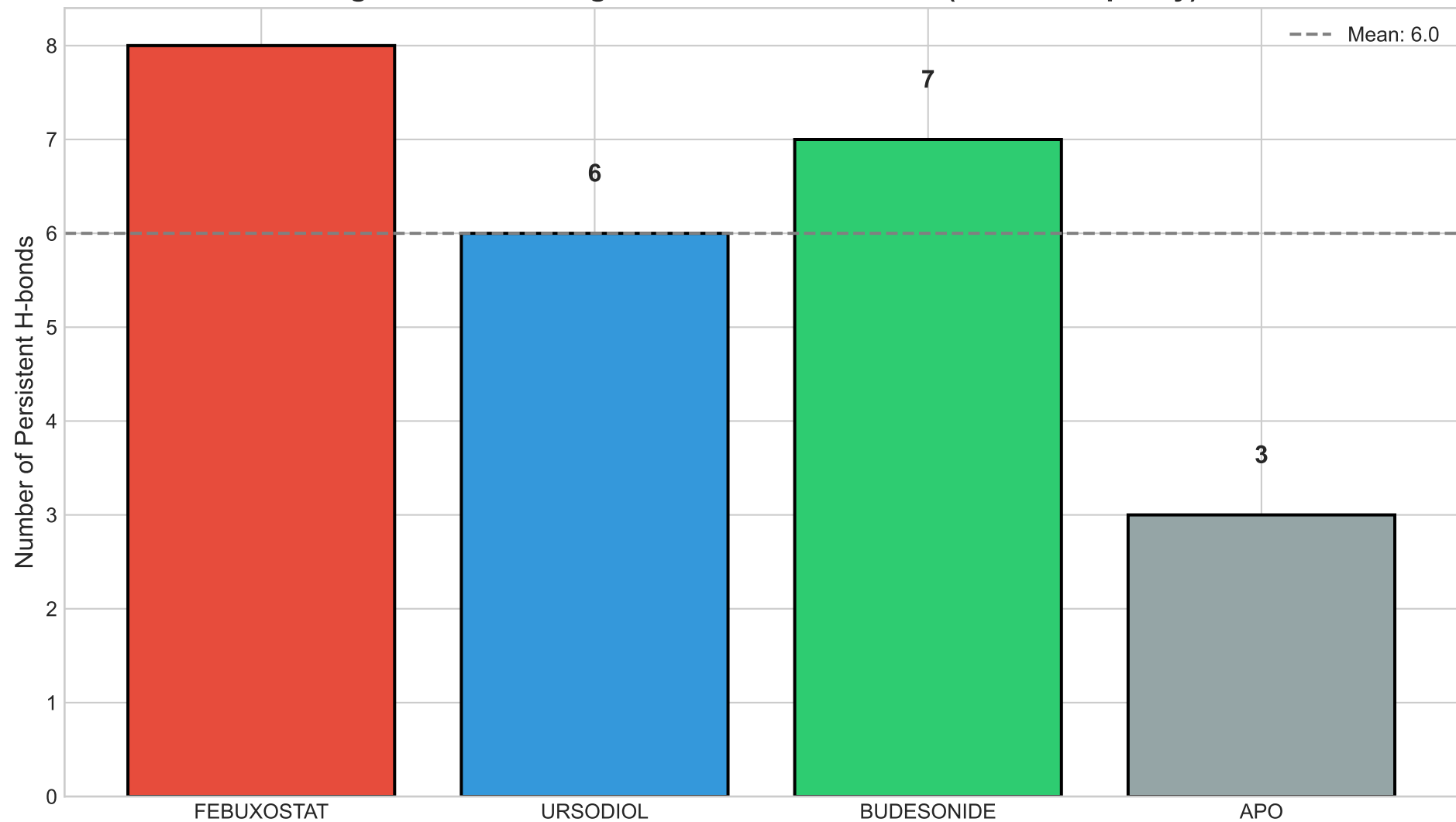
8 Figure 3: Protein-Ligand H-bond Persistence (>30% occupancy)
