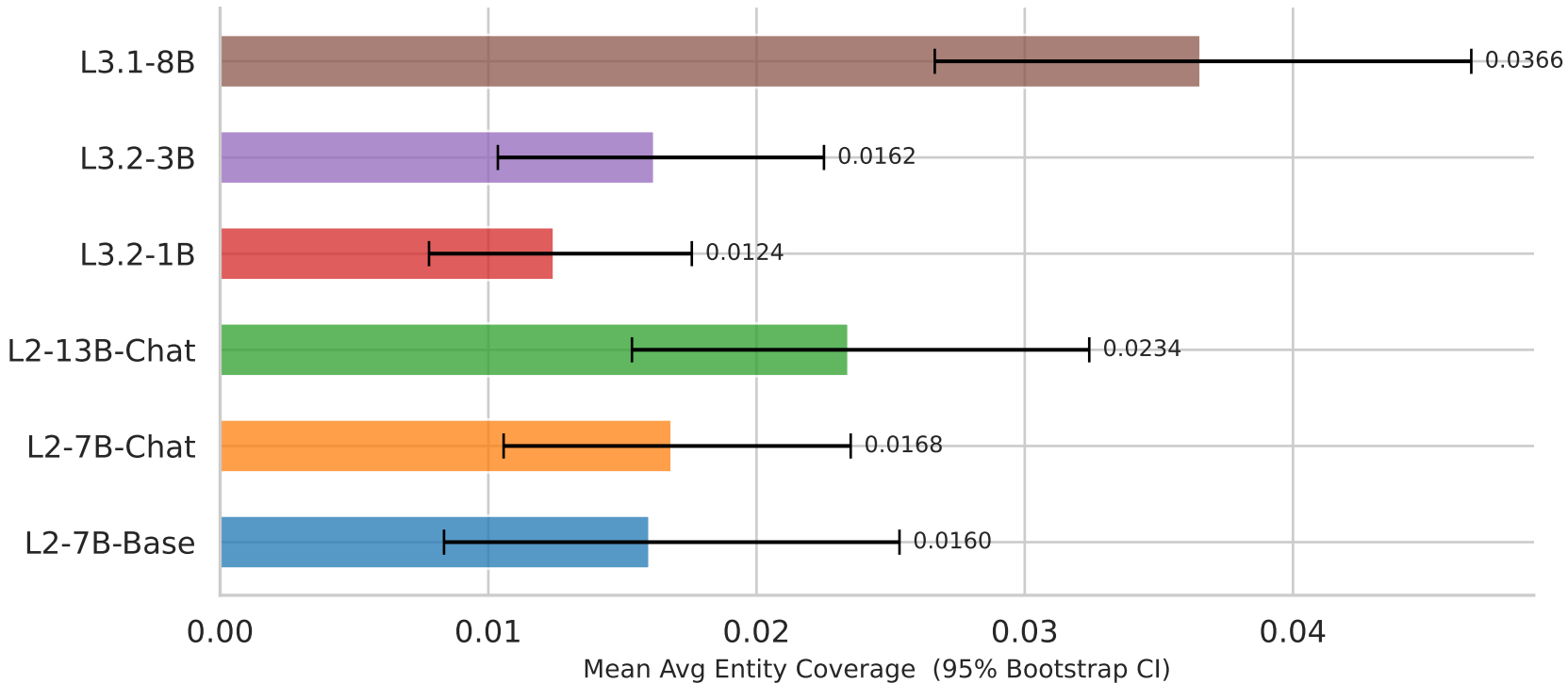
Fig S5 — Bootstrap CIs on Mean Entity Coverage per Model (error bars = 95% CI; all means significantly > 0)
