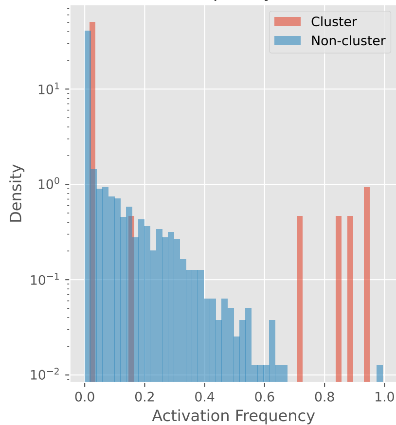
Activation Frequency Distribution
