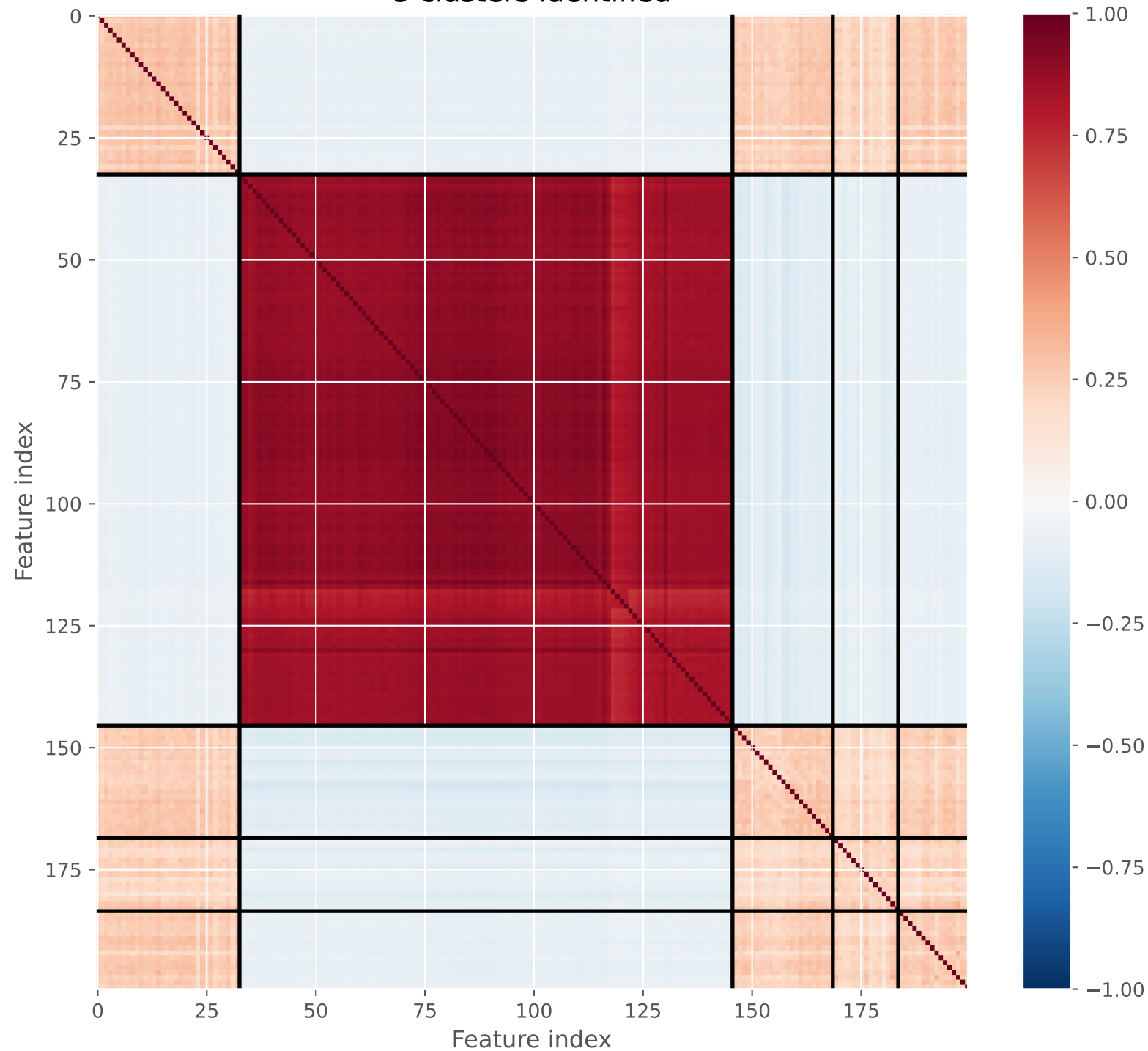
High Cooccurrence Feature Clusters 5 clusters identified
