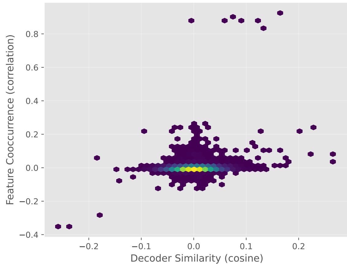
Similarity vs Cooccurrence
