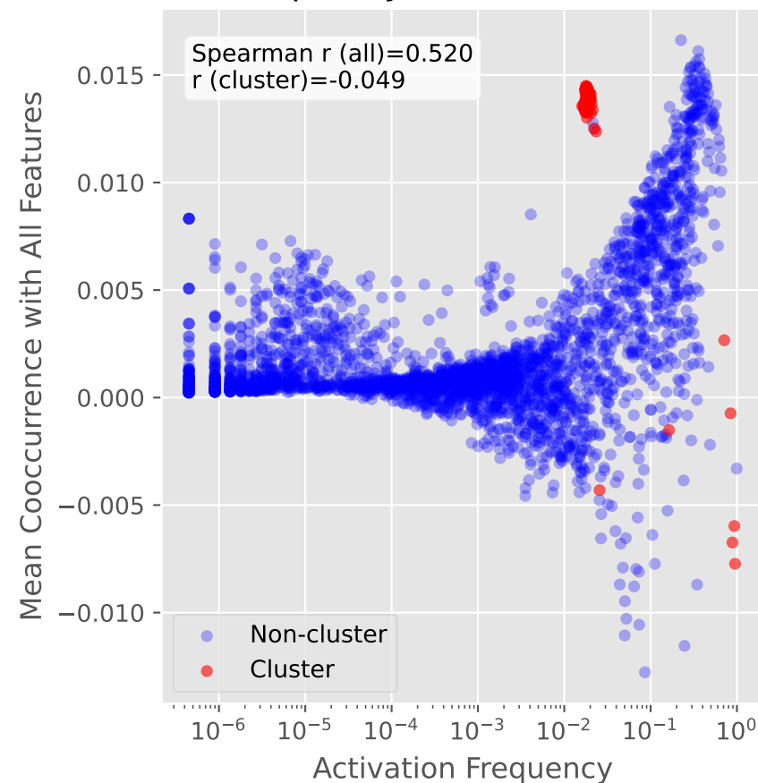
Frequency vs Cooccurrence
