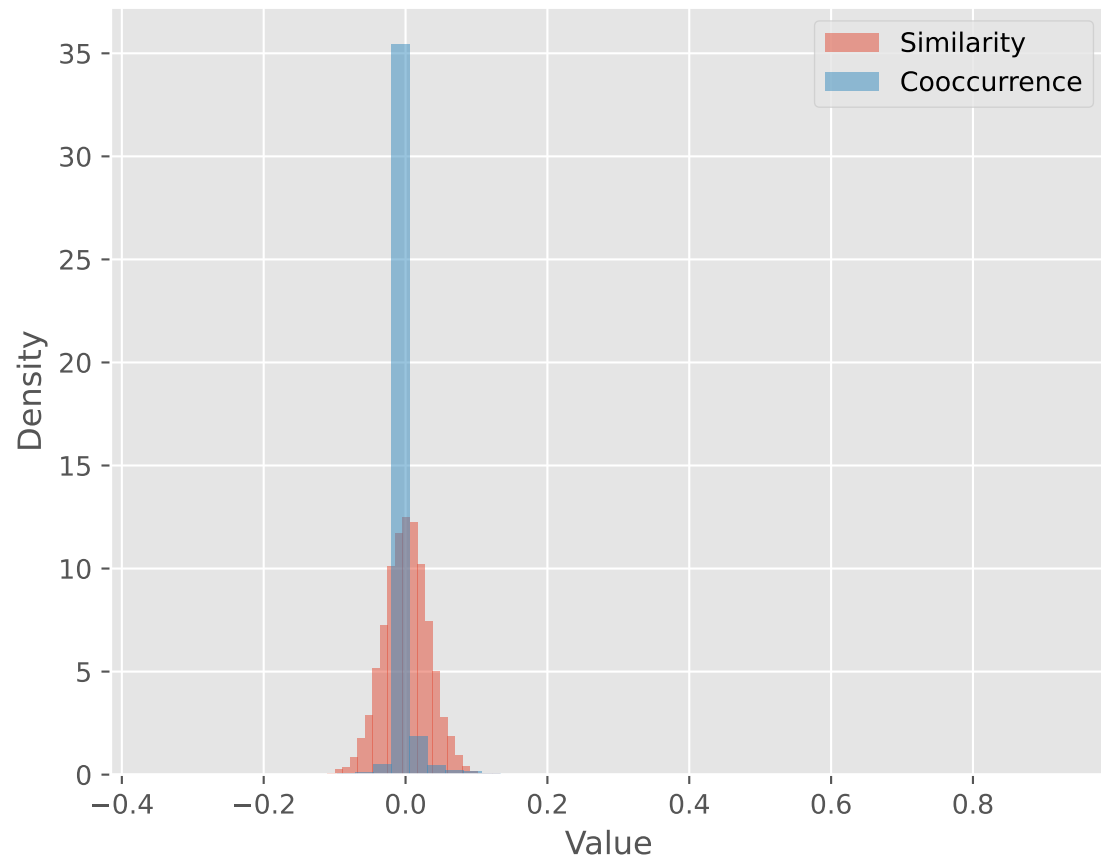
Value Distributions
