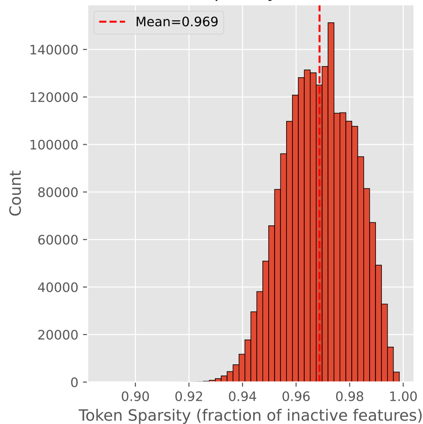
Per-Token Sparsity Distribution
