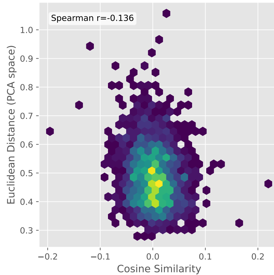
Similarity vs PCA Distance
