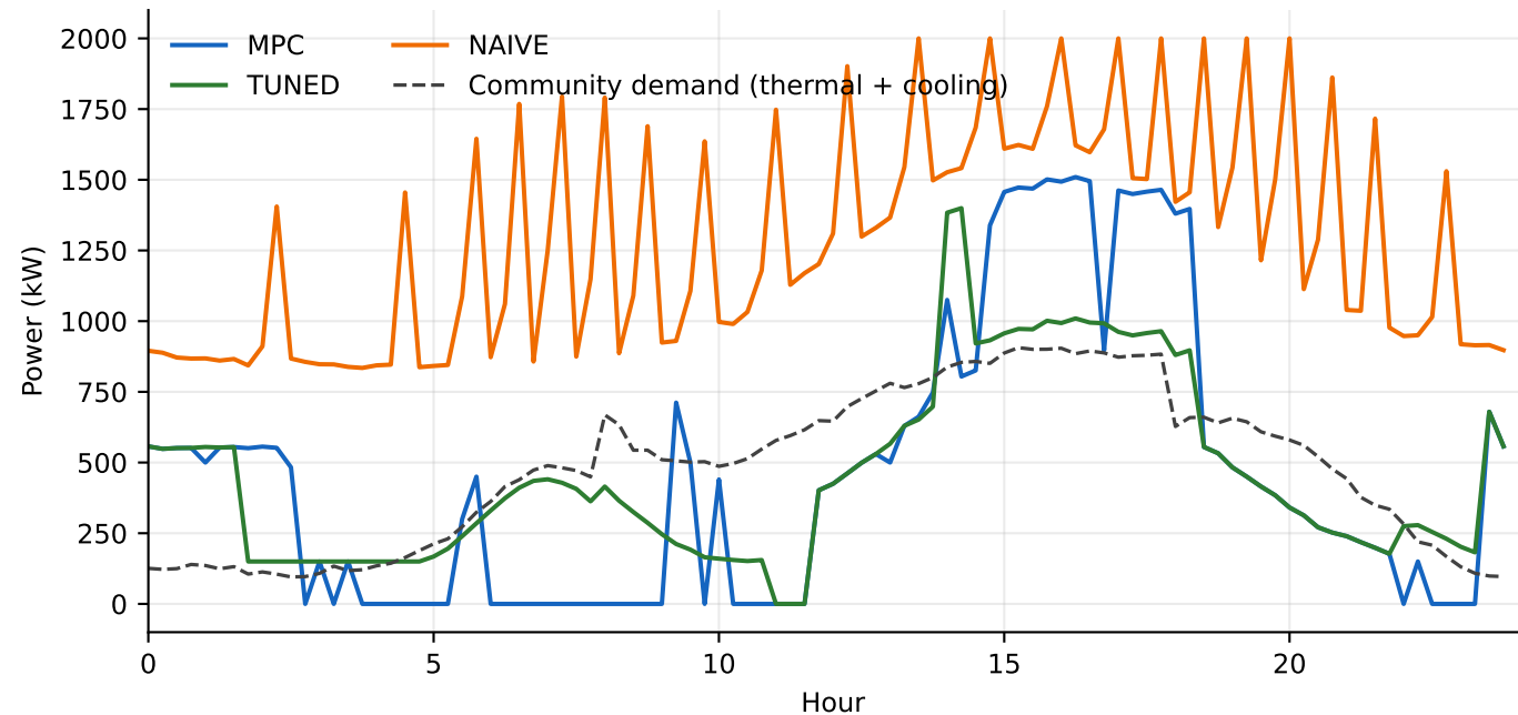
Representative 24-hour dispatch — Scenario A, seed 0
