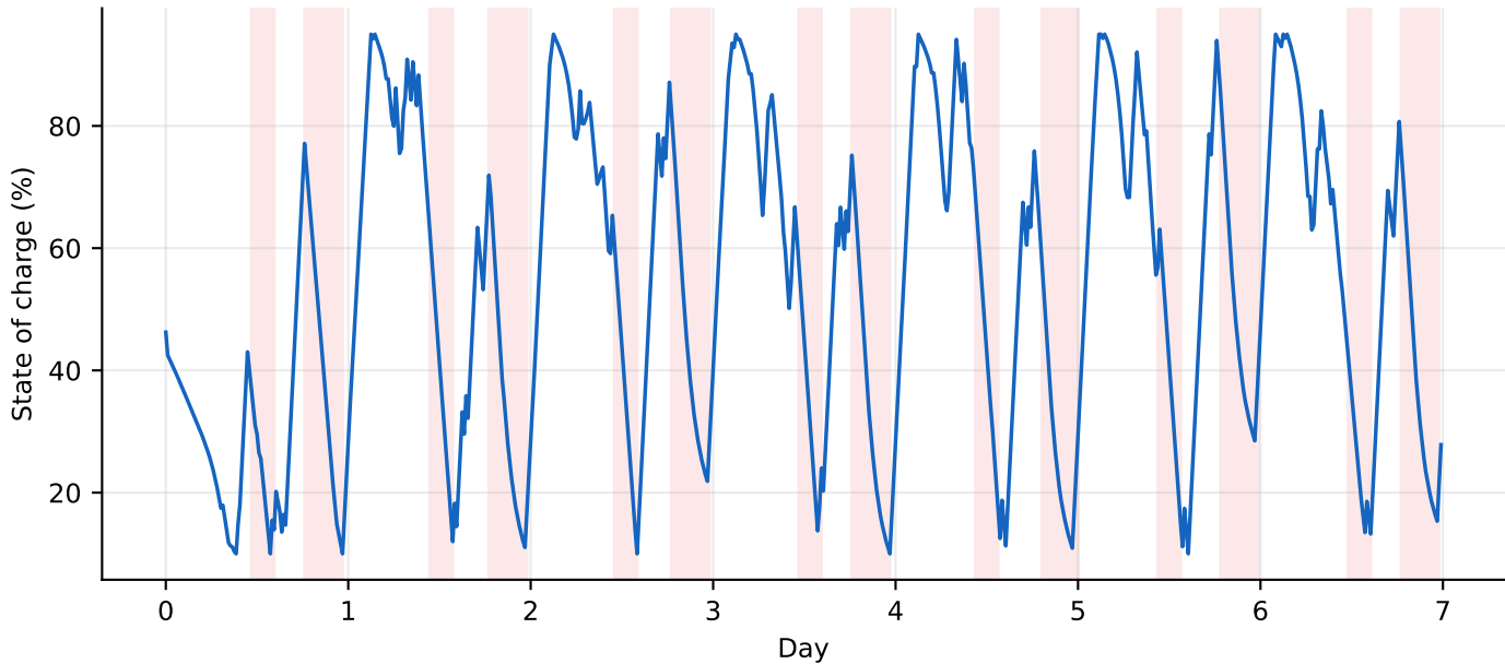
MPC thermal-store operation; outages shaded
